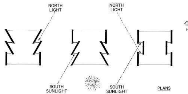
Figure A. 3: Shifting eastern and western windows to face north and south. Image derived from Lechner (2009)
