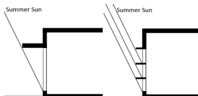
Figure A. 15: Reducing the depth of the required window's overhang via using multiple horizontal louvers.
