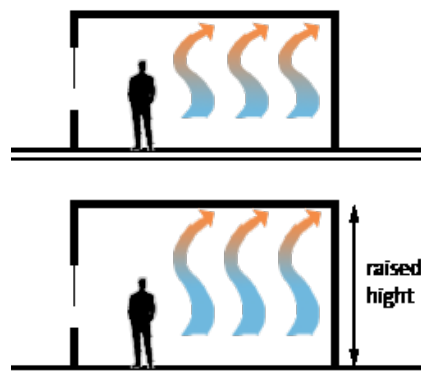
Figure A. 10: The effect of increasing the zone's height in reducing the temperature at the lower levels.
