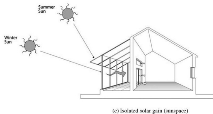
Figure A. 5: An example of an adjacent sunny space for isolated solar gains. Image source: http://what-when-how.com/energy-engineering/solar-thermal-technologies-energy-engineering/
