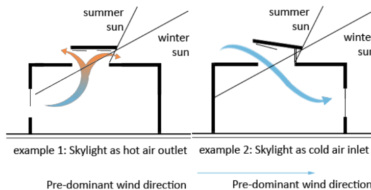
Figure A. 11: Using skylights to promote stack ventilation in hot conditions, and as a source of direct solar gains in cooler conditions.
