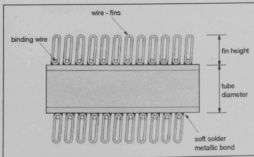
Figure 6.6: Wire Finning
