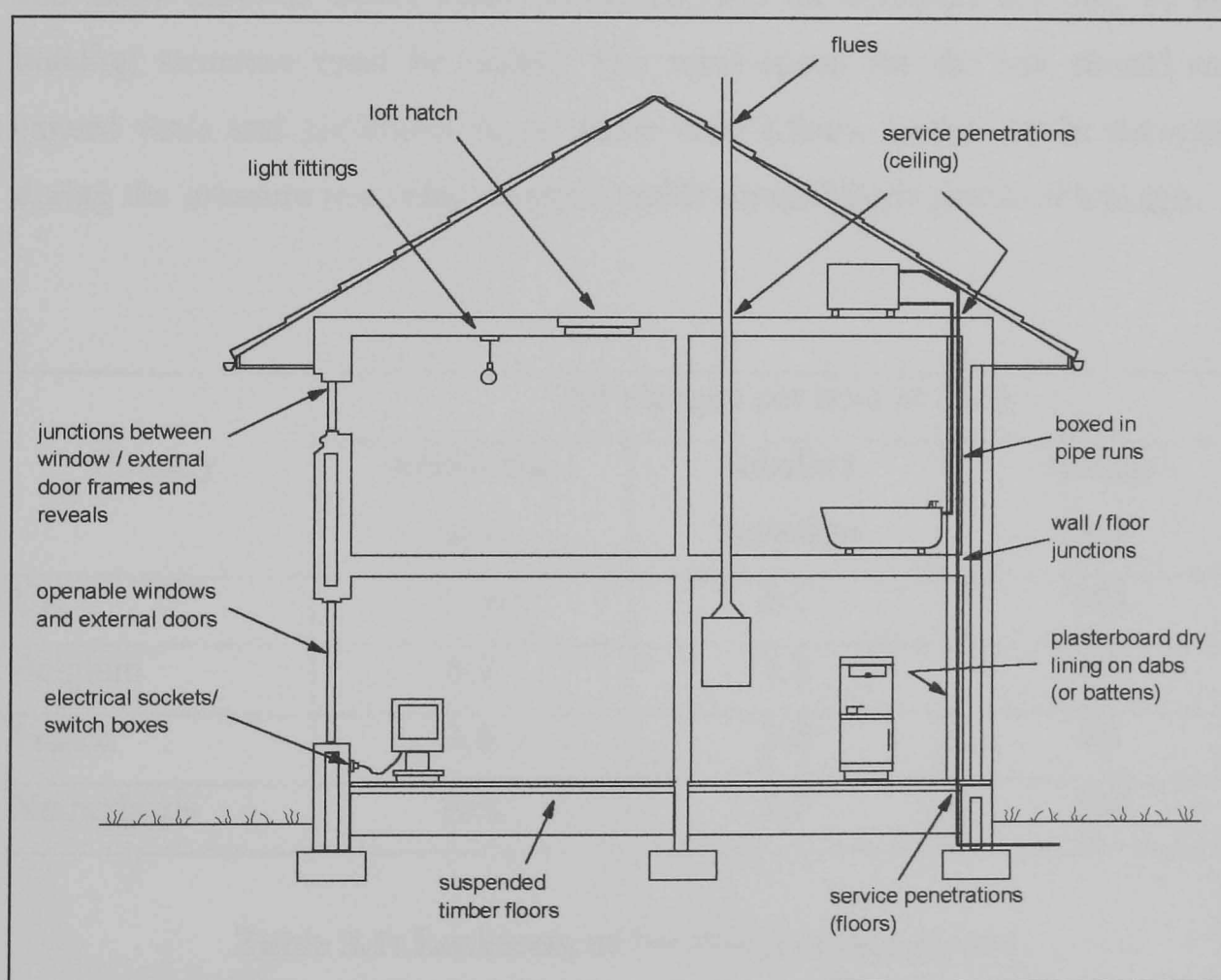
Figure 3.9: Air Leakage Routes
