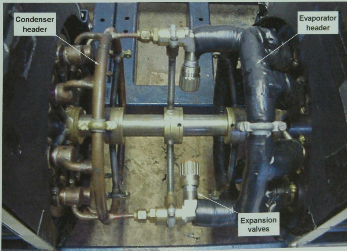
Photograph 8.3: Evaporator/Condenser Headers
