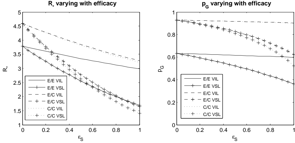
Figure 2.5: R_* and p_G varying with \varepsilon_S in VIL ( \varepsilon_L = 0 ) and VSL ( \varepsilon_L = \varepsilon_S ) cases for different latent/infectious period distributions.
