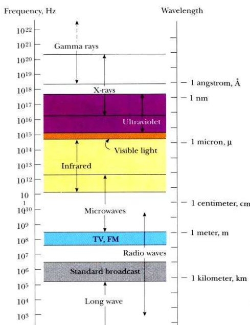
Figure 2.1 The electromagnetic spectrum (Serway, 1996).
