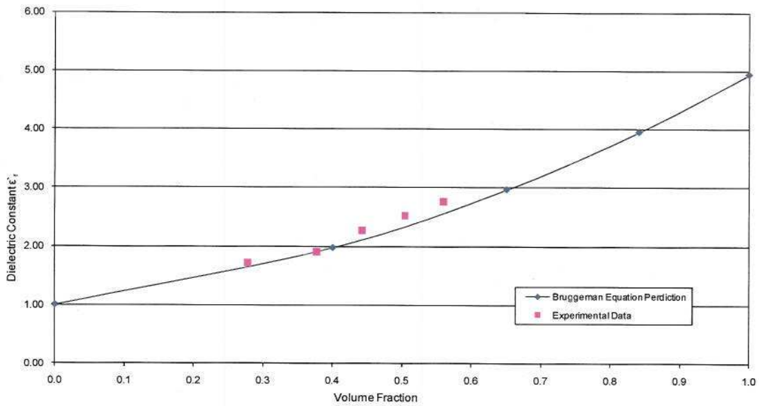
Figure 5.14 Prediction of the Dielectric Constant of Heterogeneous Mixtures according to the Bruggeman model. Experimental Data taken for Daw Mill coal at 911MHz.
