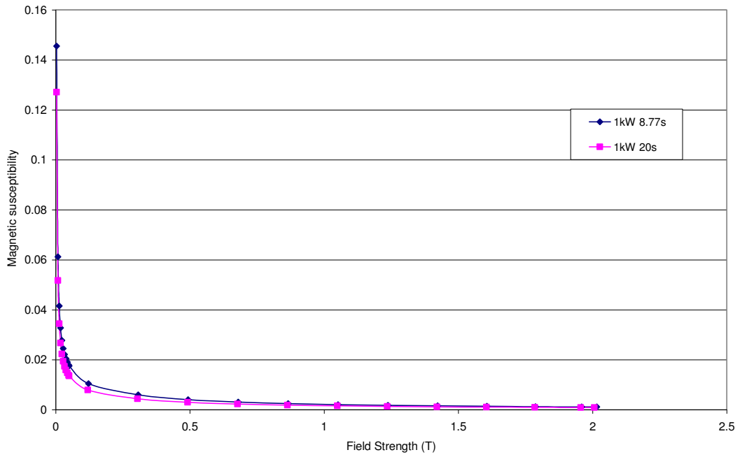
Figure 4.53 Magnetic susceptibility curves for microwave heated +425 \mu\text{m} pyrite samples.
