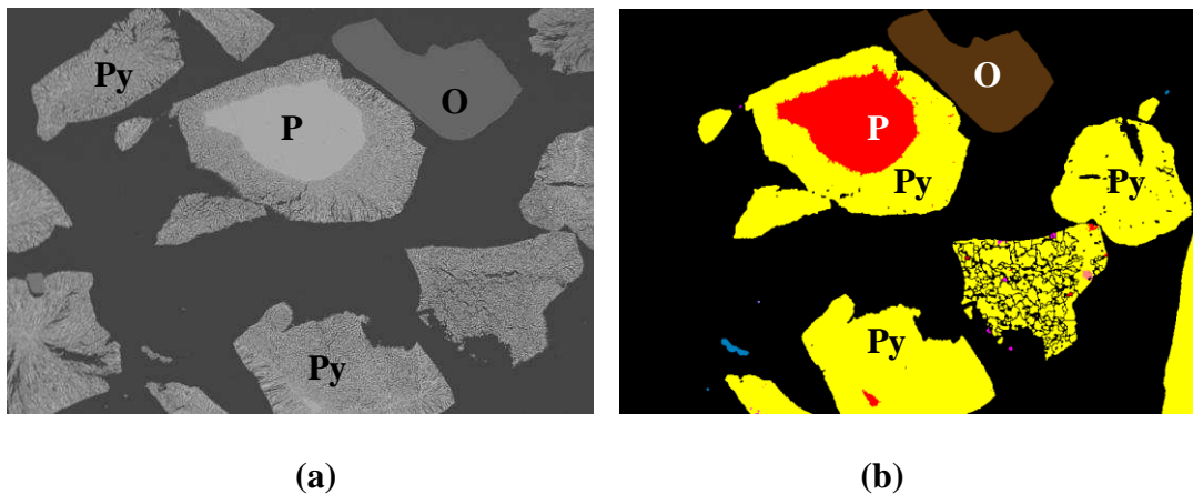
Figure 4.37 (a) BSE image showing pyrite particles +425 \mu m conventionally roasted for 15min. (b) BSE false coloured image of “a” showing areas of pyrite and pyrrhotite formation due to oxidation. (P=Pyrite, Py=Pyrrhotite, O=Other)
