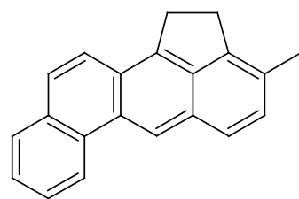
3-methylcholanthrene (3MC)
