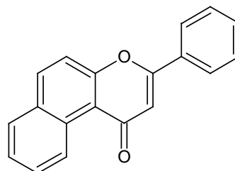
\beta -naphthoflavone
