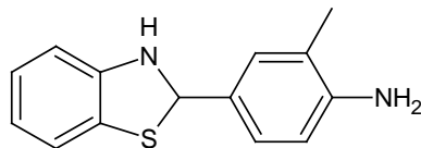
2-(4-amino-3-methylphenyl)benzothiazole (AMB)
