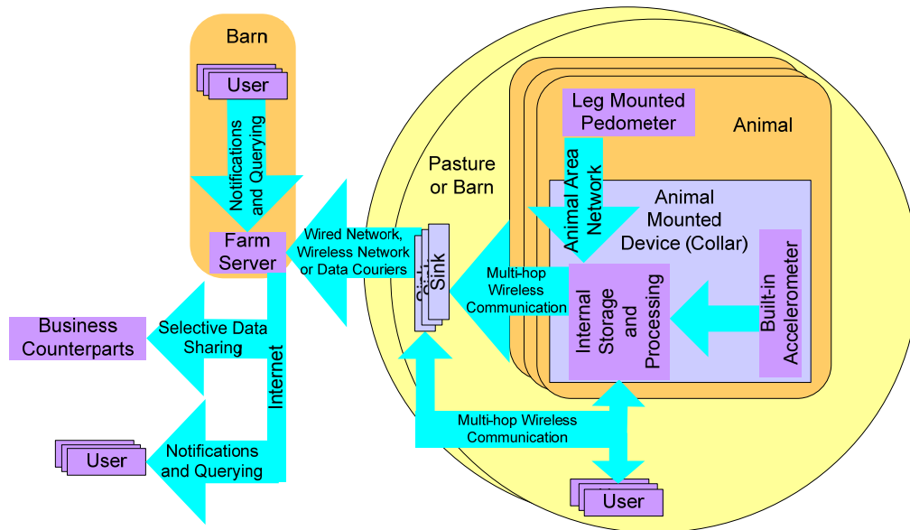
Figure 4.3. Architecture of the cattle monitoring system
