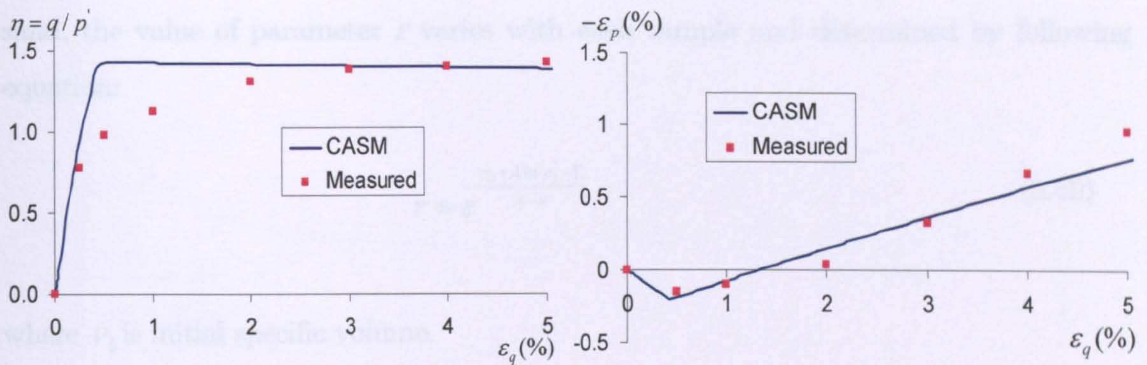
Figure 5.19 Drained compression of D662
