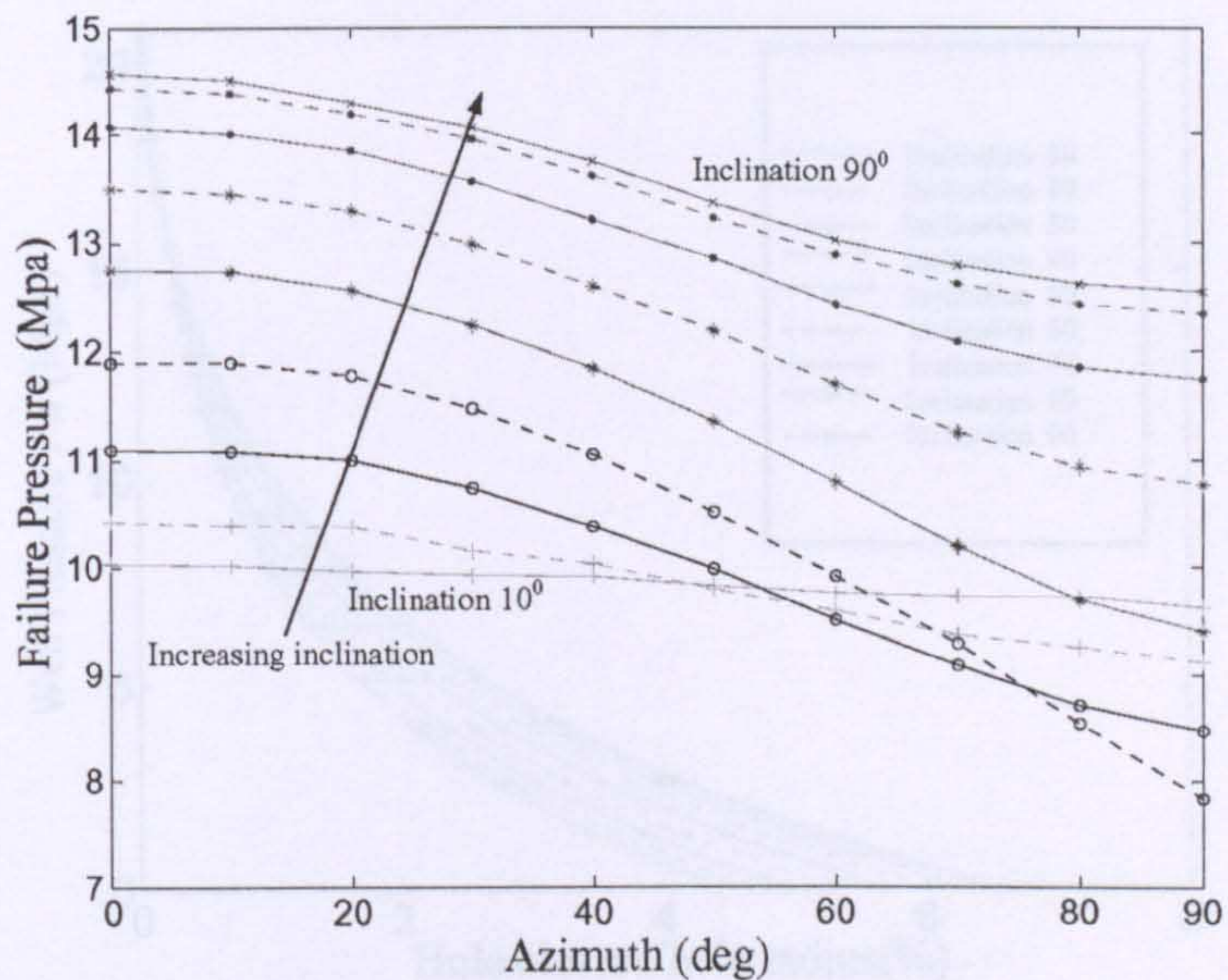
Figure 4.13 Failure Pressure according to P1 vs wellbore azimuth and various inclinations
