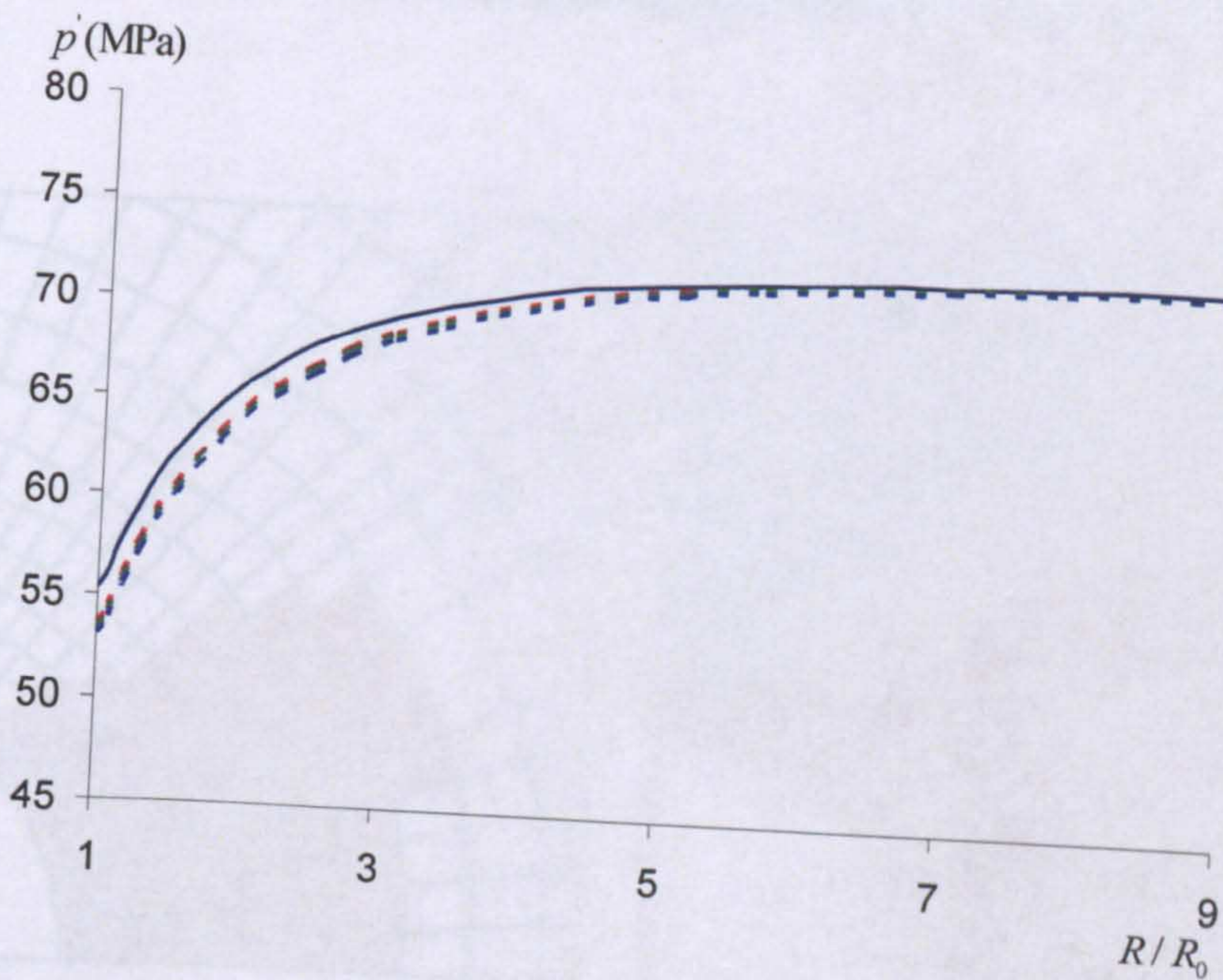
Figure 6.23 (a) Radial stress, \sigma_{rr} , (MPa) vs R/R_0 around the wellbore at the plasticity limit.
