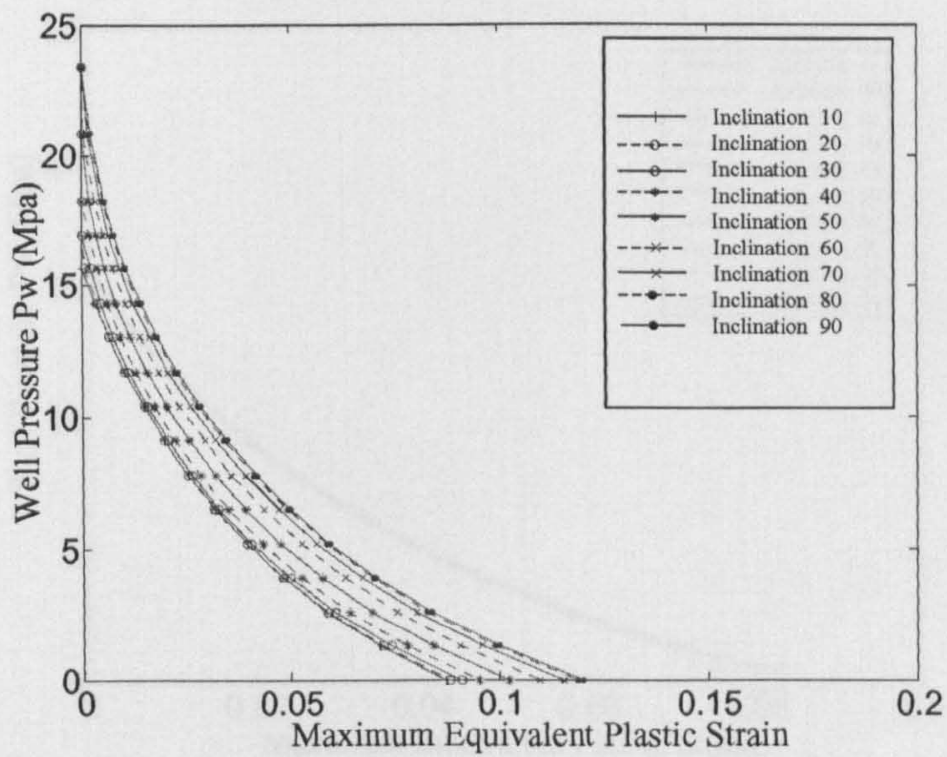
Figure 4.22 Well pressure vs maximum equivalent plastic strain for 50^\circ azimuth and various inclinations
