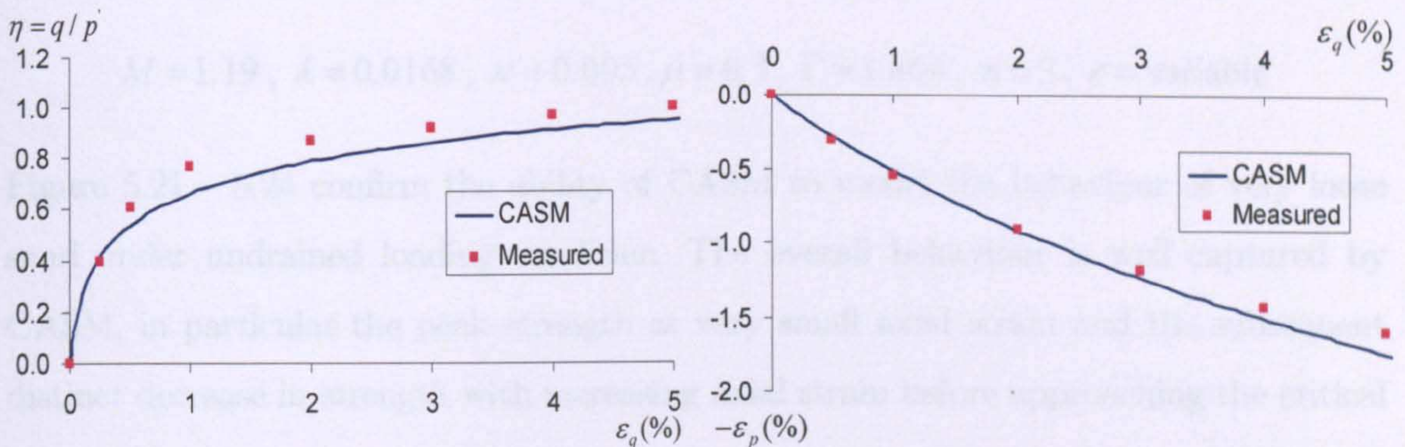
Figure 5.20 Drained compression of D684
