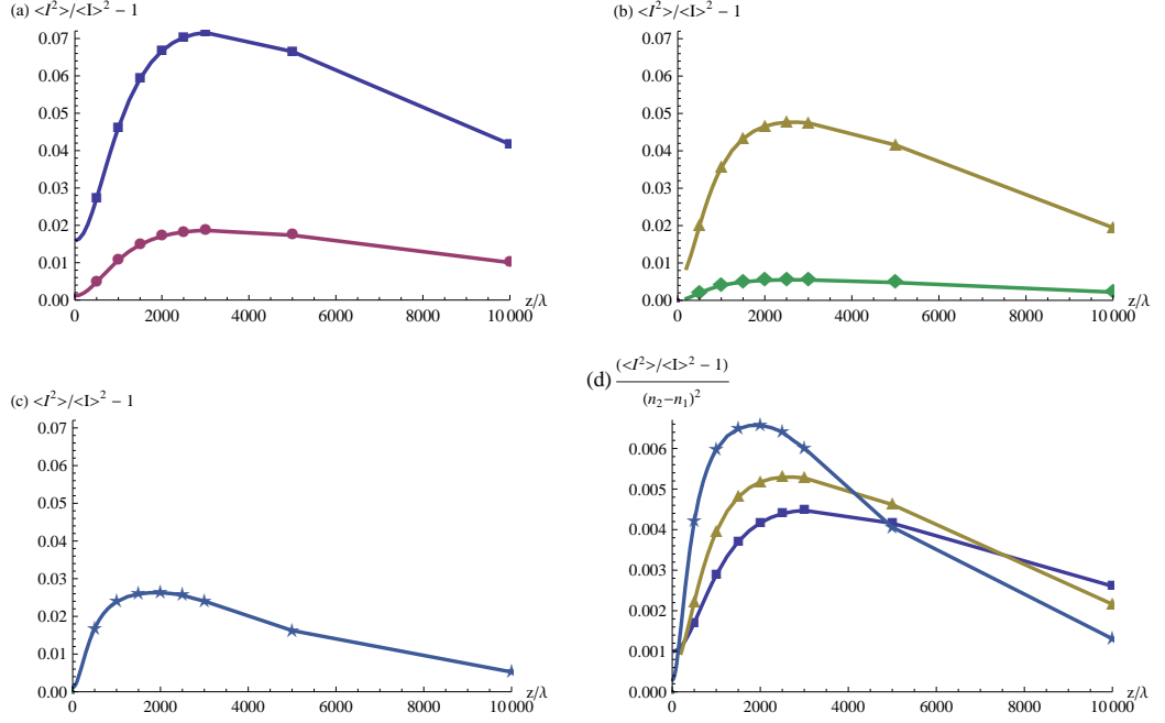
Figure 5.2: Scintillation index for the total field against optical depth into the second medium with \ell = 10\lambda and \sigma = 0.0125\lambda for the cases of (a) n_2 = -3 (dark blue squares) and 3 (purple circle); (b) n_2 = -2 (yellow triangles) and 2 (green diamonds); (c) n_2 = -1 (light blue stars). (d) shows the Scintillation index with a multiplicative factor of (n_2 - n_1)^{-2} , with this normalization the cases of n_2 = -3 and 3 become indistinguishable (dark blue squares) as do the cases of n_2 = -2 and 2 (yellow triangles). Also shown in (d) is the case of n = -1 (light blue stars). In all cases the marked data points are numerical evaluations of the functions involved, the curves comprising of interpolations between them.
