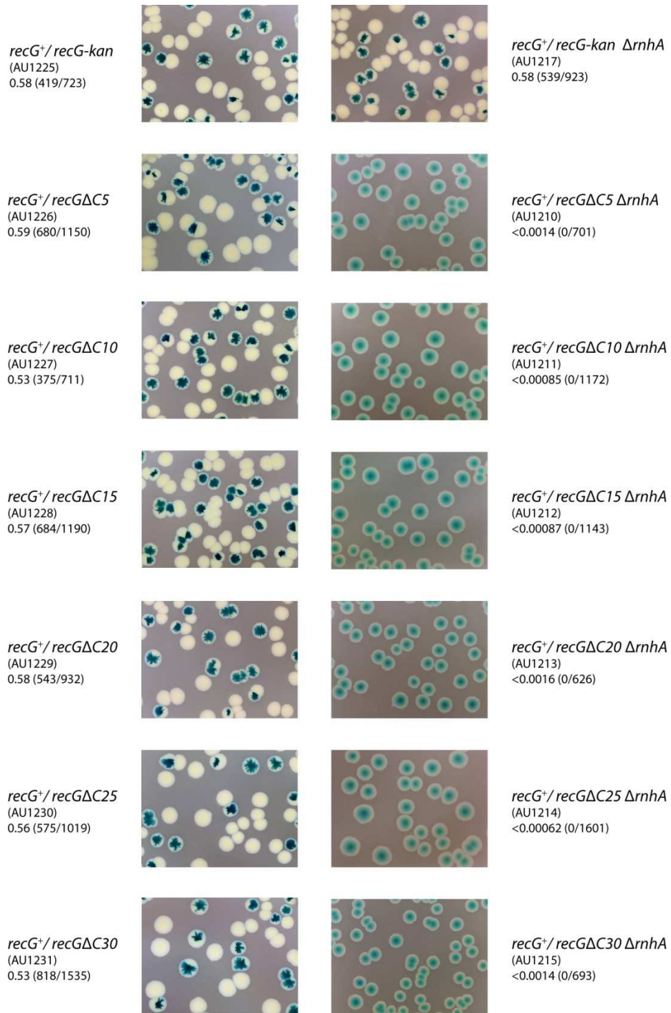
Figure 57. Deletions of the recG C-terminus are inviable when combined with \Delta rnhA . Synthetic lethality assays demonstrating the inviability of recG \Delta C5 \Delta rnhA , recG \Delta C10 \Delta rnhA , recG \Delta C15 \Delta rnhA , recG \Delta C20 \Delta rnhA , recG \Delta C25 \Delta rnhA and recG \Delta C30 \Delta rnhA . The relevant genotype is shown above each image, along with the strain number. The fraction of white colonies is shown below each image, with the number of white colonies/total colonies analysed in parentheses.
