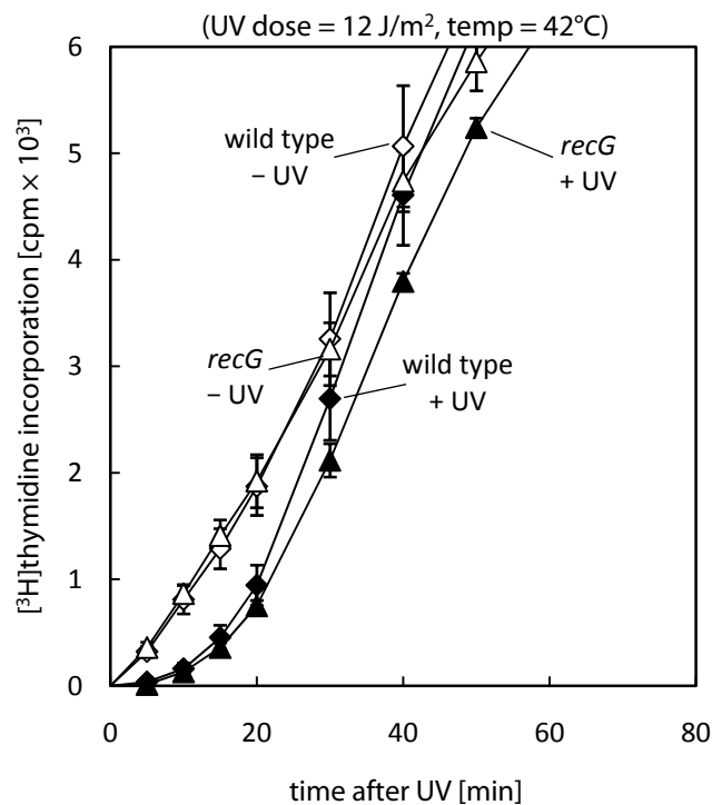
Figure 29. Effect of UV on DNA synthesis in recG cells. [ 3 H]thymidine incorporation in wild type (N1141) and recG (AU1106) cells. Data for recG are the mean ( \pm SE) of three experiments. The data for the wild type are reproduced from Figure 13 for comparison.
