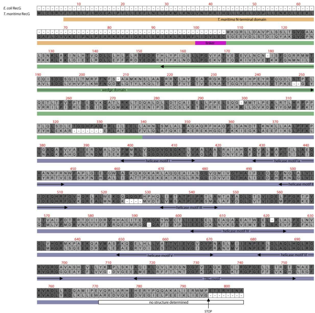
Figure 54. Amino acid sequence alignment of Escherichia coli and Thermotoga maritima RecG. The level of shading indicates percent identity (darker shaded residues have a higher percent identity). The colour coding corresponds to that used in Figure 37. Key functional domains have been labelled (Lloyd and Sharples 1991; Mahdi et al. 2003; Briggs et al. 2005). Alignment produced using clustalW.
