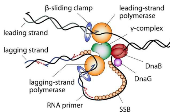
Figure 2. The E. coli replisome complex.
