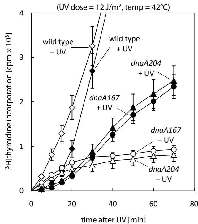
Figure 16. Effect of UV on DNA synthesis in dnaA strains. [ 3 H]thymidine incorporation in wild type (N1141), dnaA167 (AU1093), and dnaA204 (AU1094) cells. Data are the mean ( \pm SE) of three to four experiments. The data for the wild type are reproduced from Figure 13 for comparison.
