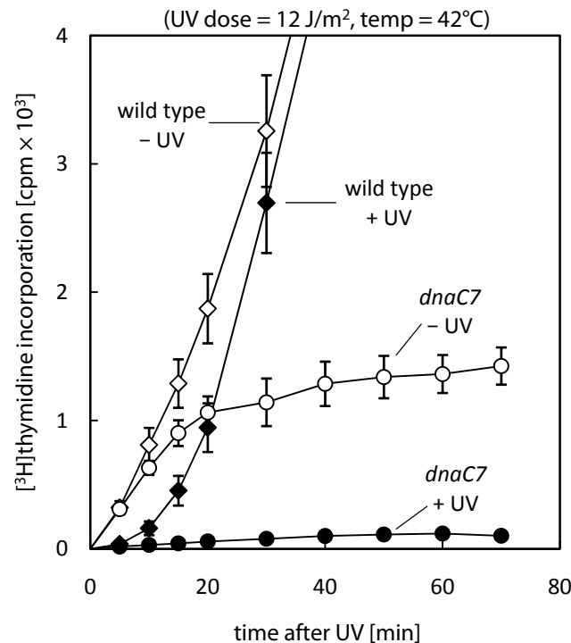
Figure 20. Effect of UV on DNA synthesis in dnaC7 strains. [ 3 H]thymidine incorporation in wild type (N1141) and dnaC7 (AU1080) cells. Data are the mean ( \pm SE) of three experiments. The data for the wild type are reproduced from Figure 13 for comparison.
