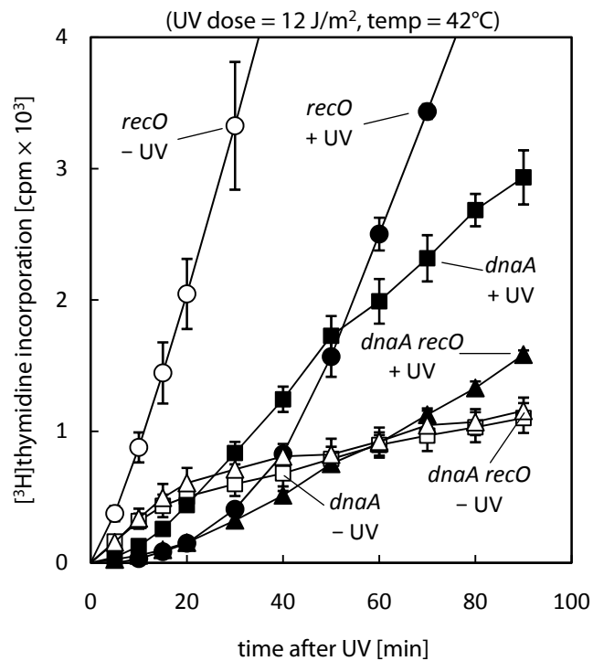
Figure 26. UV-induced synthesis is delayed in recO cells. [ 3 H]thymidine incorporation in recO (AU1110), dnaA46 (AU1068) and dnaA46 recO (AU1112) cells. Data for dnaA46 recO cells are the mean ( \pm SE) of three experiments. The data for the recO (Figure 25) and dnaA46 (Figure 15) are reproduced for comparison.
