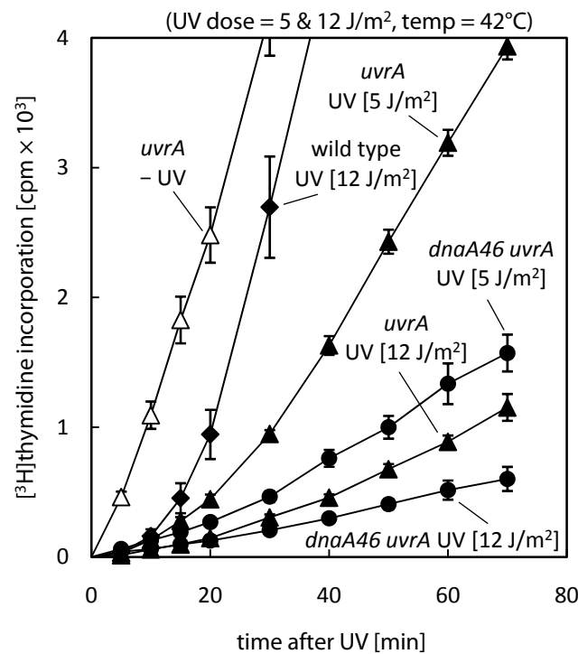
Figure 19. Changing the UV dose affects uvrA strains. [ 3 H]thymidine incorporation in wild type (N1141), uvrA (AU1075) and dnaA46 uvrA (AU1072). Data for uvrA (5 J/m 2 ) are the mean ( \pm SE) of three experiments. All other data are reproduced from Figure 17 and Figure 18 for comparison.
