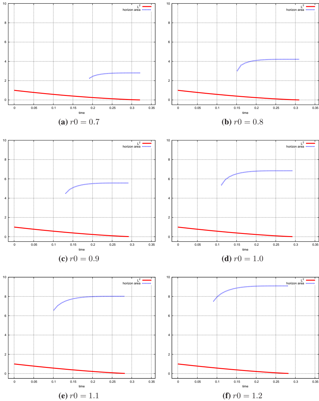
Figure 3.7: The effect of changing the value of r_0 while keeping \dot{L}_0 = 2.3
