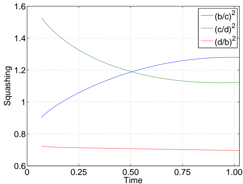
Figure 4.2: The squashing values of (what was initially) the resolved conifold, seen to be converging in time. Note the slow change to the squashing (d/b) due to the initial condition (4.20)
