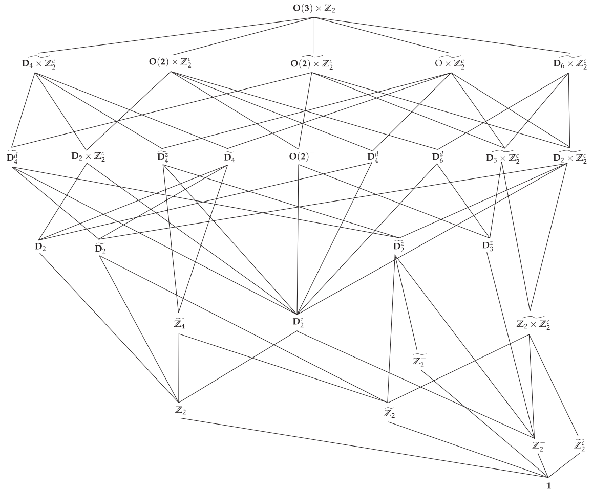
Figure 6.5: Lattice of isotropy subgroups of \mathbf{O}(3) \times \mathbf{Z}_2 for the (2,3) mode interaction.
