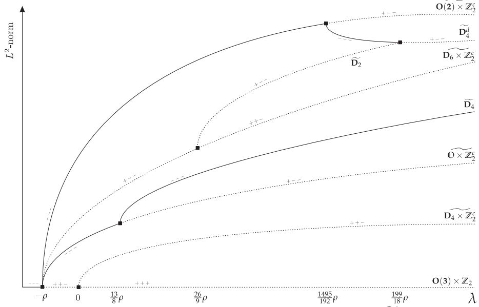
Figure 7.9: Bifurcation diagram for the Swift-Hohenberg equation in \text{Fix}(\widetilde{D}_2) for the representation on V_2 \oplus V_3 when \rho > 0 . We find that the solution with the symmetry group of a one-armed spiral, \widetilde{D}_2 , is unstable where it exists. The solution with the symmetry group of a two-armed spiral, \widetilde{D}_4 , is always stable. All bifurcations are pitchfork bifurcations. Note that the L^2 norm of the solution x = (a, b, c) is given by \|x\|^2 = a^2 + b^2 + c^2 . The diagram is not to scale but the relative sizes of the L^2 norms are shown.
