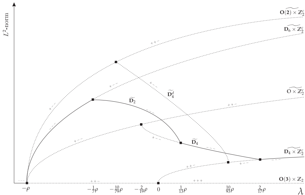
Figure 7.7: Bifurcation diagram for the system (7.2.13)–(7.2.15) when \rho > 0 . The branch of solutions with \widetilde{\mathbf{D}}_2 (one-armed spiral) symmetry is always stable and the solution with \widetilde{\mathbf{D}}_4 (two-armed spiral) symmetry is stable for some values of \lambda and \rho . All bifurcations are pitchfork bifurcations. Note that the L^2 norm of the solution x = (a, b, c) is given by \|x\|^2 = a^2 + b^2 + c^2 . The diagram is not to scale but the relative sizes of the L^2 norms are shown.
