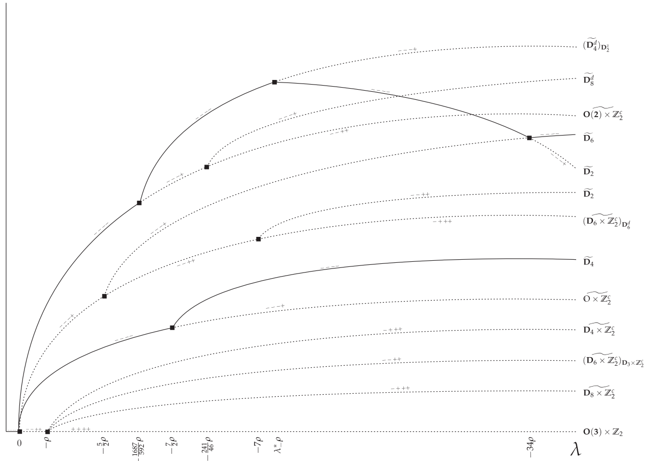
Figure 7.16: Bifurcation diagram for the Swift–Hohenberg equation in \text{Fix}(\widetilde{\mathbf{D}}_2) for the representation on V_3 \oplus V_4 when \rho < 0 . All bifurcations are pitchfork bifurcations with the exception of the bifurcation at \lambda = -34\rho which is transcritical.
