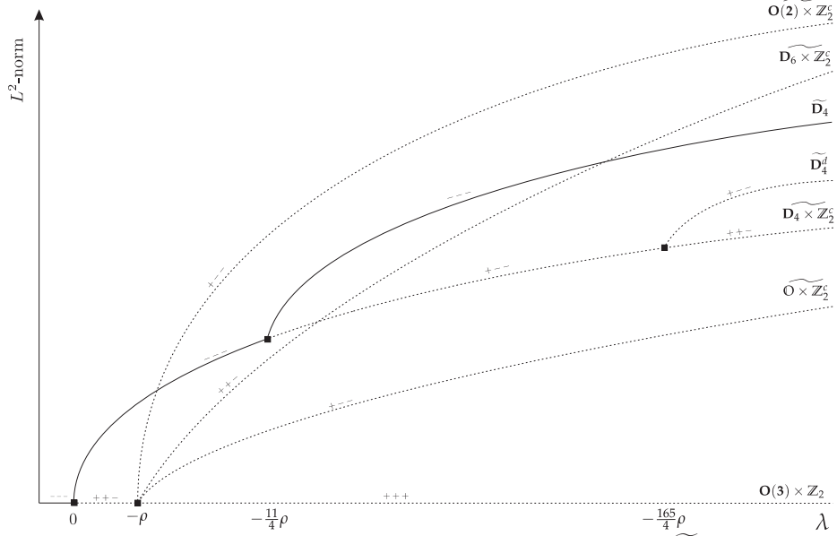
Figure 7.10: Bifurcation diagram for the Swift-Hohenberg equation in \text{Fix}(\widetilde{D}_2) for the representation on V_2 \oplus V_3 when \rho < 0 . We find that the solution with the symmetry group of a one-armed spiral, \widetilde{D}_2 , does not exist but a stable solution with \widetilde{D}_4 does exist when \lambda > -\frac{11}{4}\rho and is always stable. All bifurcations are pitchfork bifurcations. Note that the L^2 norm of the solution x = (a, b, c) is given by \|x\|^2 = a^2 + b^2 + c^2 . The diagram is not to scale but the relative sizes of the L^2 norms are shown.
