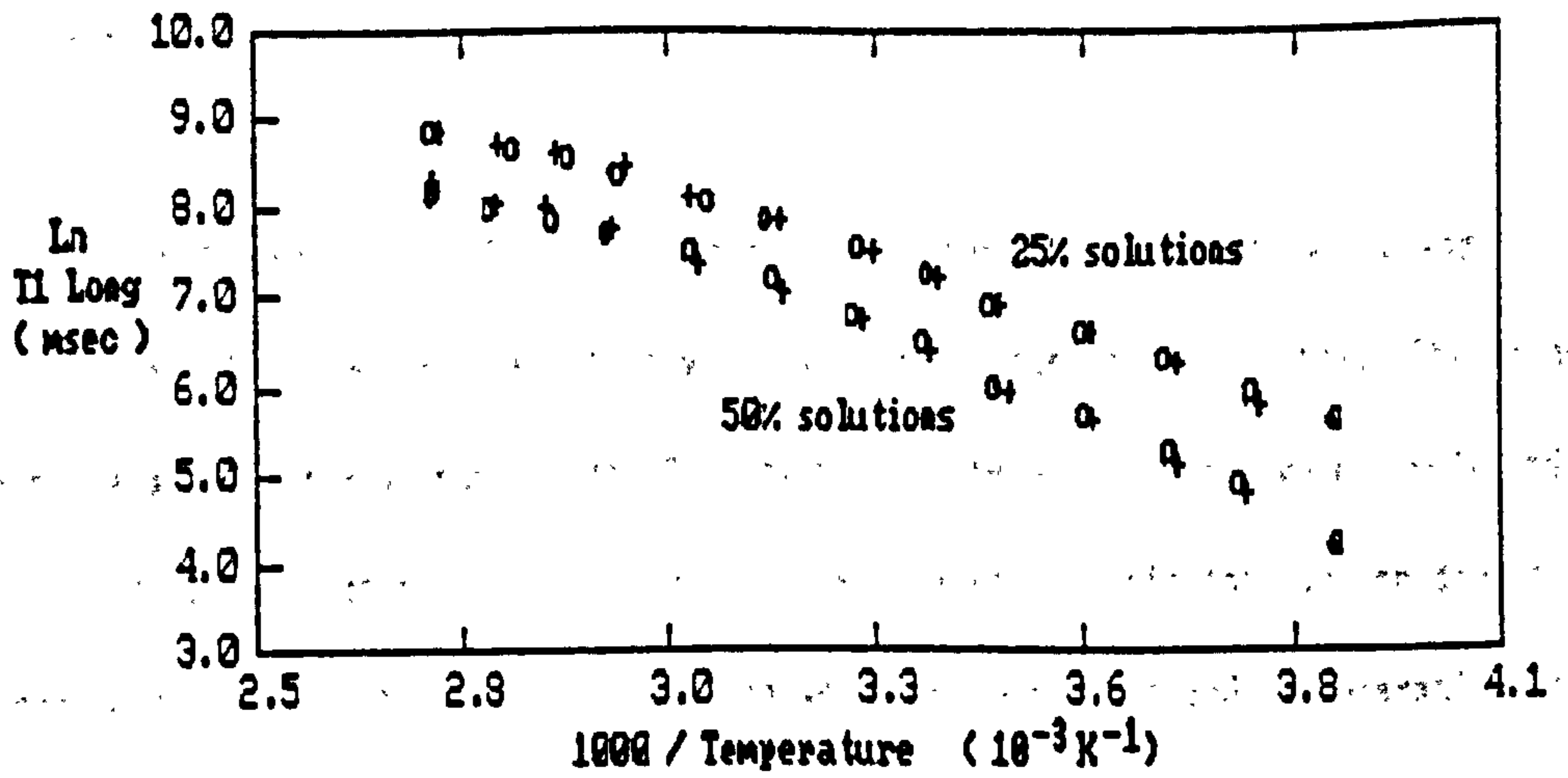
Figure 6.26a Spin-lattice relaxation in 25% and 50% solutions of PEG 1000 (o), and PEG 20,000 (+) as a function of temperature. Long ( \text{H}_2\text{O} ) component.
