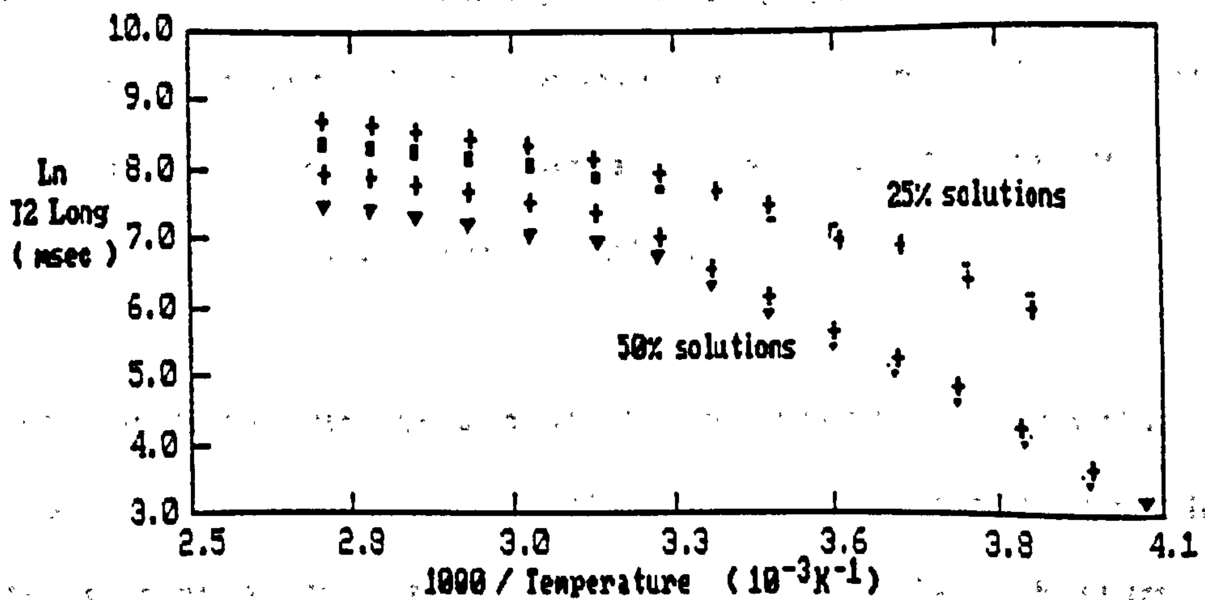
Figure 6.26b Spin-spin relaxation in 25% and 50% solutions of PEG 1000 (+), 4000 (o), and 20,000 ( \nabla ) as a function of temperature. Long ( \text{H}_2\text{O} ) component.
