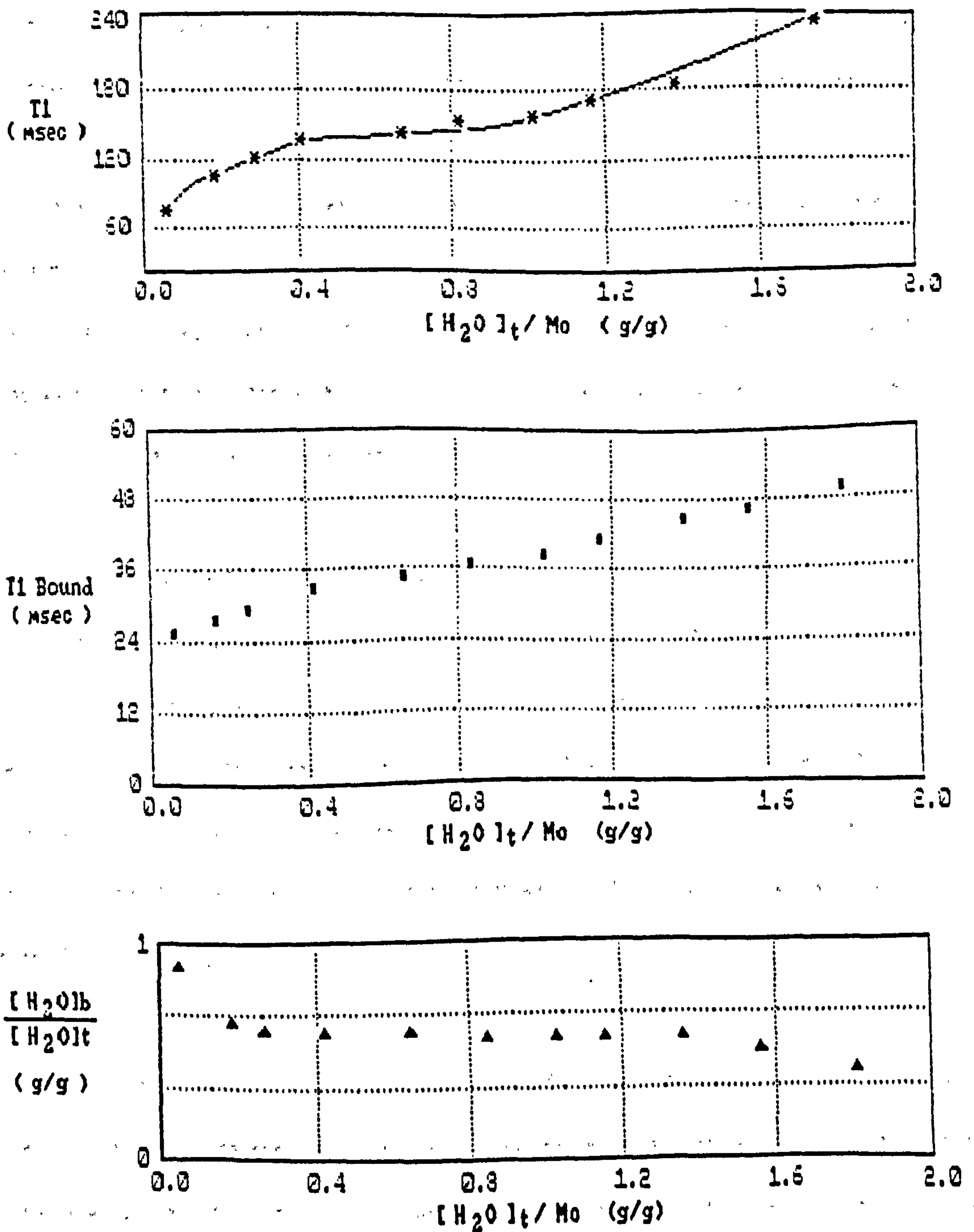
Figure 6.10 Theoretical changes in T_1 bound (■) and [H_2O]_b/[H_2O]_t (▲) for birch heartwood, used to predict nature of T_1 observed (*).
