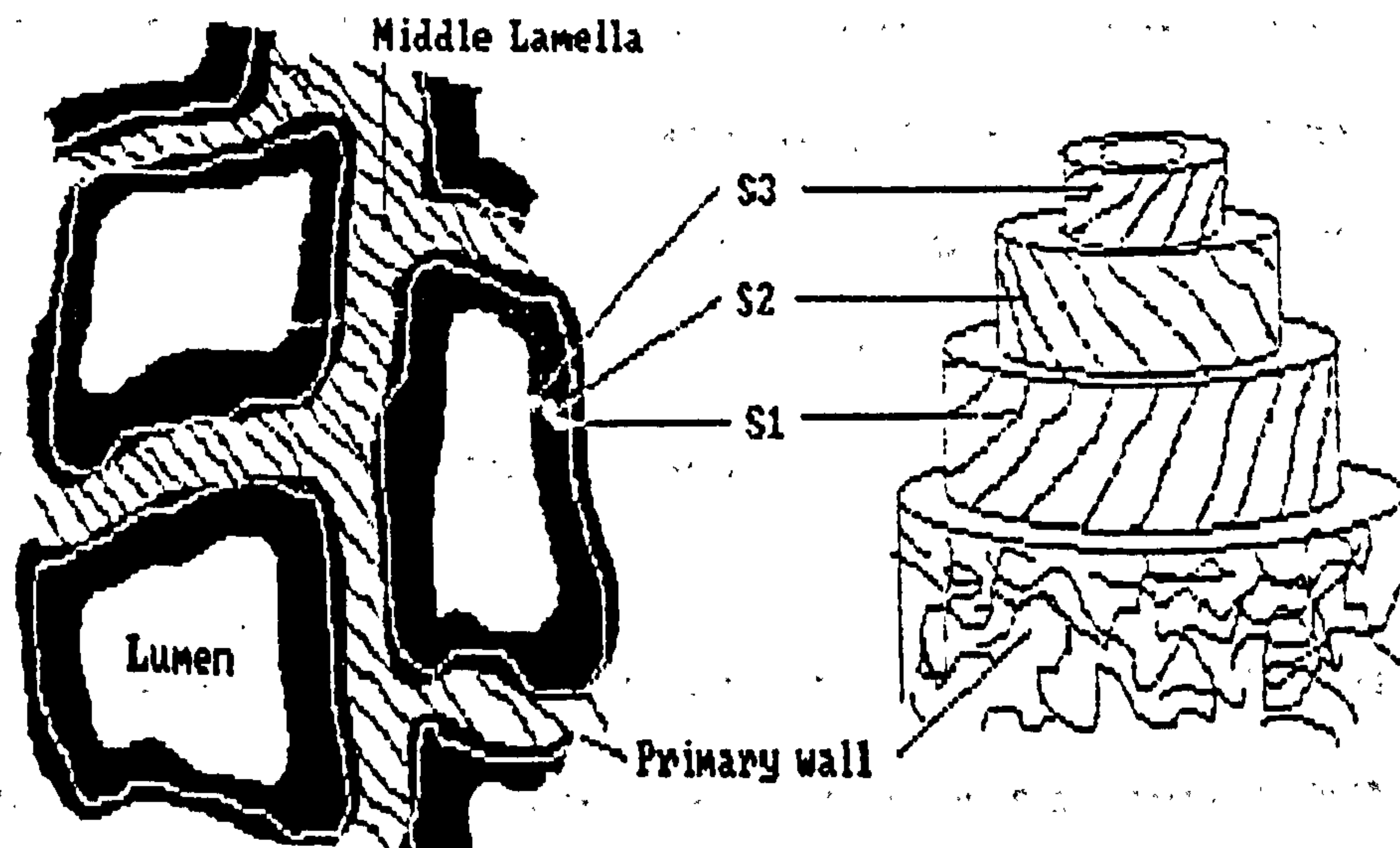
Figure 2.1 Organisation of cell walls in wood fibres.
