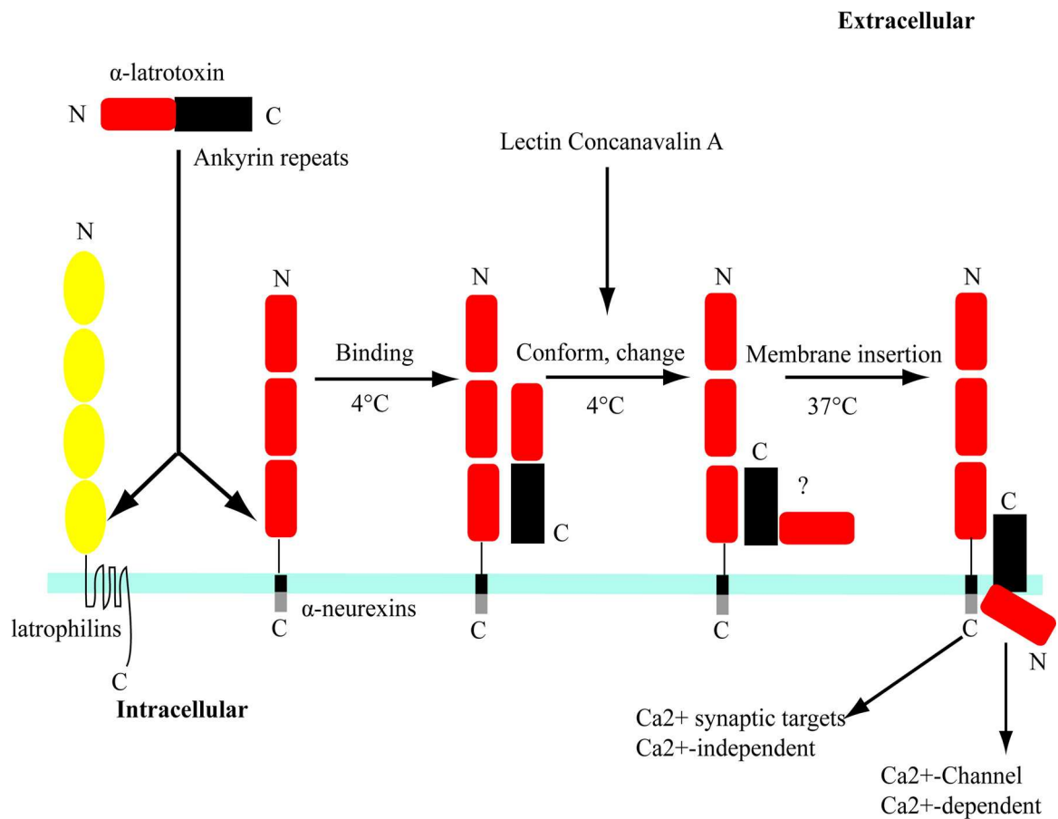
Figure 1.2 Model of the latrophilin or neurexin binding to \alpha -latrotoxin . Latrophilin binds to \alpha -latrotoxin or neurexin; there is then a conformational change occurs at 4°C which stimulates membrane insertion that needs higher temperature. The presence of lectin concanavalin A is involved in conformational change but does not prevent binding of receptor. \text{Ca}^{2+} channel formation and translocation into the presynaptic intracellular space occur from membrane insertion triggering two processes of exocytosis. N and C represent N-terminals and C-terminals of different proteins. Reproduced from [2].
