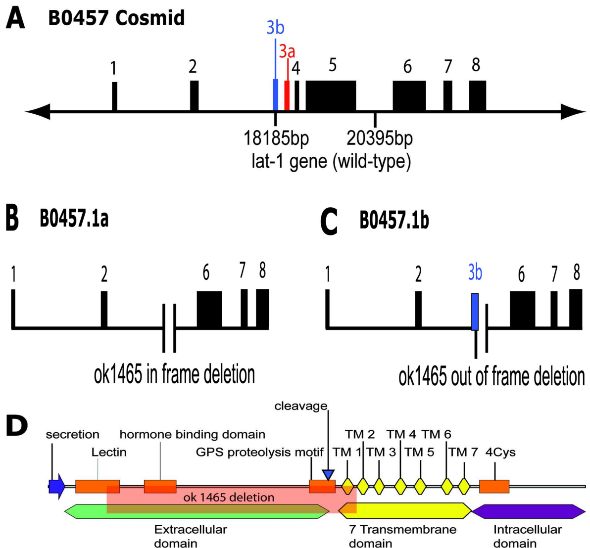
Figure 3.2 The ok1465 lat-1 allele. A The top picture shows a cartoon of the lat-1 gene (wild-type) in the B0457 cosmid, lat-1 ok1465 allele deletion spans nucleotides 18185-20395 between exon 3b and exon 5. Exons 1-8 of lat-1 gene (wild-type) are depicted in black boxes apart from 3a and 3b which are depicted in red and blue respectively, introns are indicated as black lines. B , C The middle pictures show cartoons of the lat-1 ok1465 gene. B The splice variant of lat-1 ok1465 (B0457.1a) that shows in-frame deletion of exons 3-5, skipping 3b due to alternative splicing. C shows the splice variant of lat-1 ok1465 (B0457.1b) which has an out of frame deletion in the middle of exon 3b and finishes in the intron before exon 6. D The bottom picture is the predicted lat-1a protein. The picture shows putative domains of the lat-1 protein, including the secretion region (a blue arrow), the galactose-binding lection domain (Lectin), the “hormone receptor motif domain” (hormone binding domain), the G-protein coupled receptor proteolysis site (GPS proteolysis motif, with the site of cleavage indicated by a blue triangle), the transmembrane domain receptors (TM1, TM2, TM3, TM4, TM5, TM6, TM7), the area of four cysteine domain (4xCys). The position of the amino acids deleted in the ok1465 deletion is shown by a light pink box marked “ok1465 deletion”. The extracellular domains are highlighted in green colour, The seven transmembrane domains is shown in yellow colour, and the intracellular domains are C-terminal, in purple colour.
