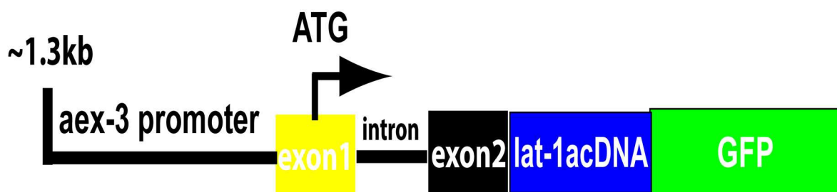
Figure 3.14 Translational reporter gene fusion of lat-1a cDNA driven by aex-3 promoter. Cartoon shows in-frame translational fusion of lat-1a cDNA to reporter gene. ~1.3kb, 5' end of aex-3 promoter contains start codon ATG (black arrow) in the middle of exon 1 (yellow) with an intron (black line) and exon 2 (black box) with lat-1a cDNA (blue box) fused to green fluorescent protein GFP (green box), resulting construct is designated as pAA409. ( see section 2.10.3)
