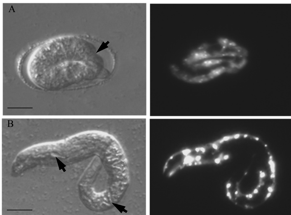
Figure 3.13 Phenotypes of TM1 lat-1a cDNA on wild-type worms. The diagram shows the photographs of arrested embryo and larvae from transgenic animal carrying N2 [ P_{1.5\text{kb } lat-1}::TM1(lat-1a \text{ cDNA})::gfp;unc-54::mCherry ] [pAA407;pAA414]. All images were captured under DIC optics and mCherry filter using the same focal point at 100x magnification. Embryos were dissected from transgenic adult hermaphrodite as described in section 2.8.1. A is a typical example of 3-fold stage arrested embryo that failed to elongate as indicated by the arrow. B is a typical example of larval 1 with the rupture of intestine and pharynx as shown by the arrow. Scale bar is 50 \mu\text{m} .
