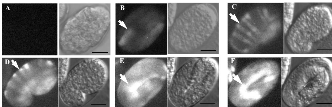
Figure 3.6 Embryonic expression pattern of lat-1::GFP . The diagram shows the photographs of different stages of embryo development of transgenic animal carrying ~1.5kb, 5' end of lat-1 fused to gfp reporter gene. Embryos were dissected from integrated lines of transgenic animals. All images were taken under GFP filter and visible DIC using the same focal point (A) embryo at 40-cell stage before GFP detection (post-fertilization) (B) GFP fluorescence was first detected at the position of gut cells (white arrow), 60 mins post-fertilization (C) a dorsal sheet of gut cells (white arrow) intercalation (D) migration of dorsal gut cells (white arrow) (E) beginning of gut cells expression at 2-fold stage with twitching (white arrow) (F) gut cells expression at 3-fold stage (white arrow). Scale bar is 25 \mu m, and all images were captured at 40x magnification.
