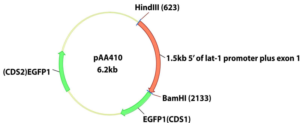
Figure 2.4 The map of lat-1::GFP construct. The map shows the transcriptional reporter fusion of ~1.5kb, 5' regulatory region of lat-1 promoter with four amino acid of exon 1 sequence. Restriction enzymes; HindIII and BamHI show their restriction sites at 623 and 2133 position respectively upon fusion to pEGFP-N1 reporter gene (green fluorescent protein; gfp ). with two coding sequences CDS 1&2 The resulting plasmid is designated as pAA410 with the size of 6.2kb
