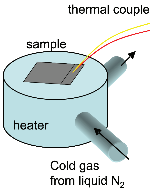
Figure 4.7: A sample and a thermocouple are mounted on the heater
