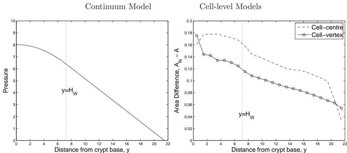
Figure 5.3: Plots showing how the compression of the cells varies with distance from the base of the crypt for (left) the continuum model, (right) the cell-centre model and the cell-vertex model. For the continuum model, the pressure, p , is plotted; for the cell-centre and cell-vertex models the difference between actual cell area, A , and natural cell area A_N , is plotted. The dotted horizontal line, y = H_W , shows the edge of the Wnt-stimulated region, where for y \leq H_W cells can proliferate and for y > H_W cells cannot.
