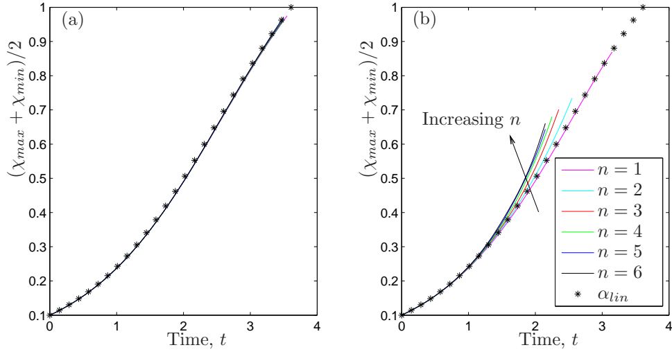
Figure 2.8: Series of plots comparing the collocation method (lines) and the analytic method (2.62) (* symbols) for the midpoint of the moving boundary between the populations of the cells, (\chi_{max} + \chi_{min})/2 . \chi_{max} , \chi_{min} represent the maximum and minimum values at any x of \chi(x, t) for each time value. The plots show how the behaviour varies for different mode numbers, n , of the initial conditions, \chi_0 = 0.1 + 0.005 \cos(nx/\beta) . Parameter values: k = 2 , \lambda_1 = 1.5 , \lambda_2 = 0 and \beta = 1 . In (a) D = 2 and in (b) D = 0.5 .
