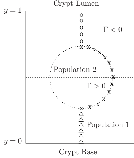
Figure 2.17: Sketch of the placements of the collocation points for two cell populations on the crypt wall. (X) marks collocation points where (2.99) and (2.100) need to be satisfied and at (O) and ( \Delta ) (2.98) needs to be satisfied.
