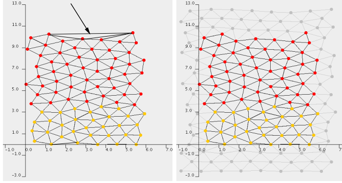
Figure 3.3: Plots showing why ghost nodes are needed at the top and bottom of the crypt. (Left) When there are no ghost cells, the Delaunay triangulation connects cells large distances away from each other, to achieve a convex hull. (Right) When there are ghost cells, large unrealistic connections are avoided.
