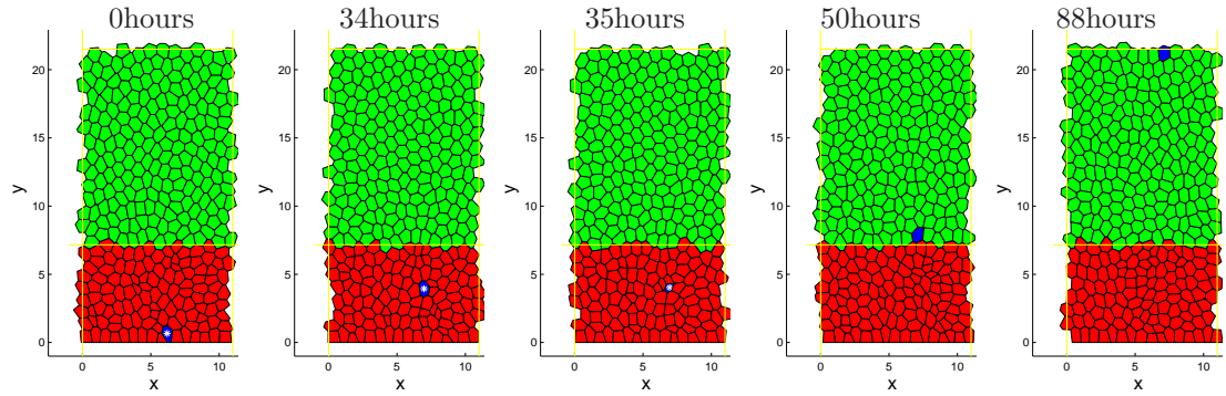
Figure 4.14: Series of plots showing a single cell (marked in blue) move throughout the crypt. Plotted for (left to right) initial position ( t = 0 ), shortly before a cell division ( t = 34 ), shortly after a cell division ( t = 35 ), shortly after the cell has moved out of the proliferative region ( t = 50 ), shortly before the cell is to be removed from the top of the crypt ( t = 88 ). Transit cells are coloured red or blue marked with a *, differentiated cells are coloured green or blue without a *. The parameter values are as stated in §B.3.
