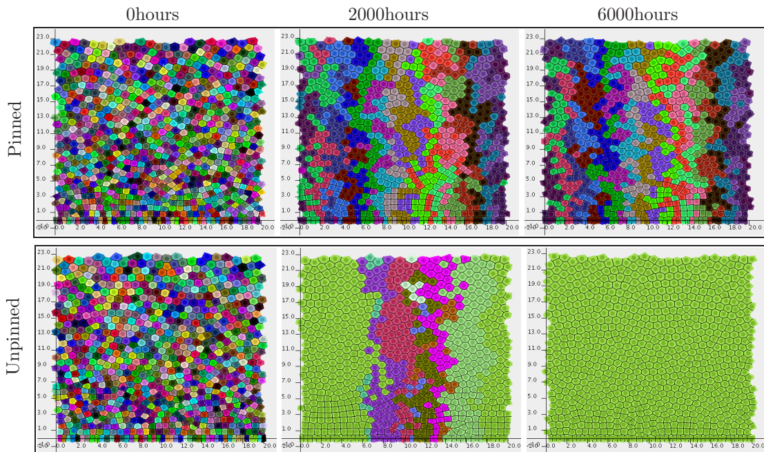
Figure 3.7: Snapshots showing how unpinning the stem cells (bottom three plots) can lead to a monoclonal crypt; this is not possible in Meineke et al. 's original model (top three plots). In the left two snapshots, initially all the cells are marked with a different colour. When a cell divides, both daughter cells retain the same colour as the parent cell. When the stem cells are pinned (top), no one lineage dominates the crypt, and the crypt's composition is similar after two thousand hours (middle top) and six thousand hours (right top), with 23 lineages in each. When the stem cells are unpinned (bottom), eventually one lineage dominates the crypt (middle bottom) and after six thousand hours the crypt becomes monoclonal (right bottom). See §A.1 for parameter values.
