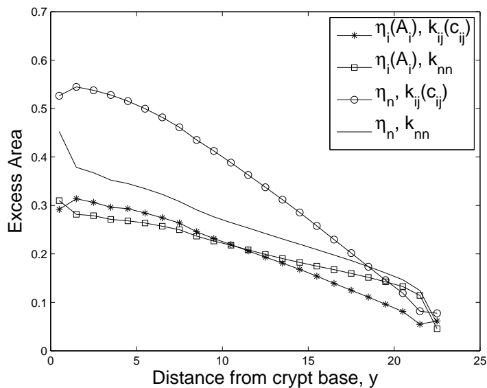
Figure 3.14: Series of plots showing how a simple measure of the compression experienced by the cells P_i (= A_N - A_i) , the difference between actual area and target area), varies within the crypt and how it depends on the mechanical properties of the cells. Each line represents different mechanical scenarios for the cells with (\eta_n, k_{nn}) constant drag and linear springs, (\eta_n, k_{ij}(c_{ij})) constant drag and edge-length dependent springs, (\eta_i(A_i), k_{nn}) area-dependent drag and linear springs and (\eta_i(A_i), k_{ij}(c_{ij})) area-dependent drag and edge-length dependent springs. In all cases, the compression decreases with distance up the crypt. See §A.1 for parameter values.
