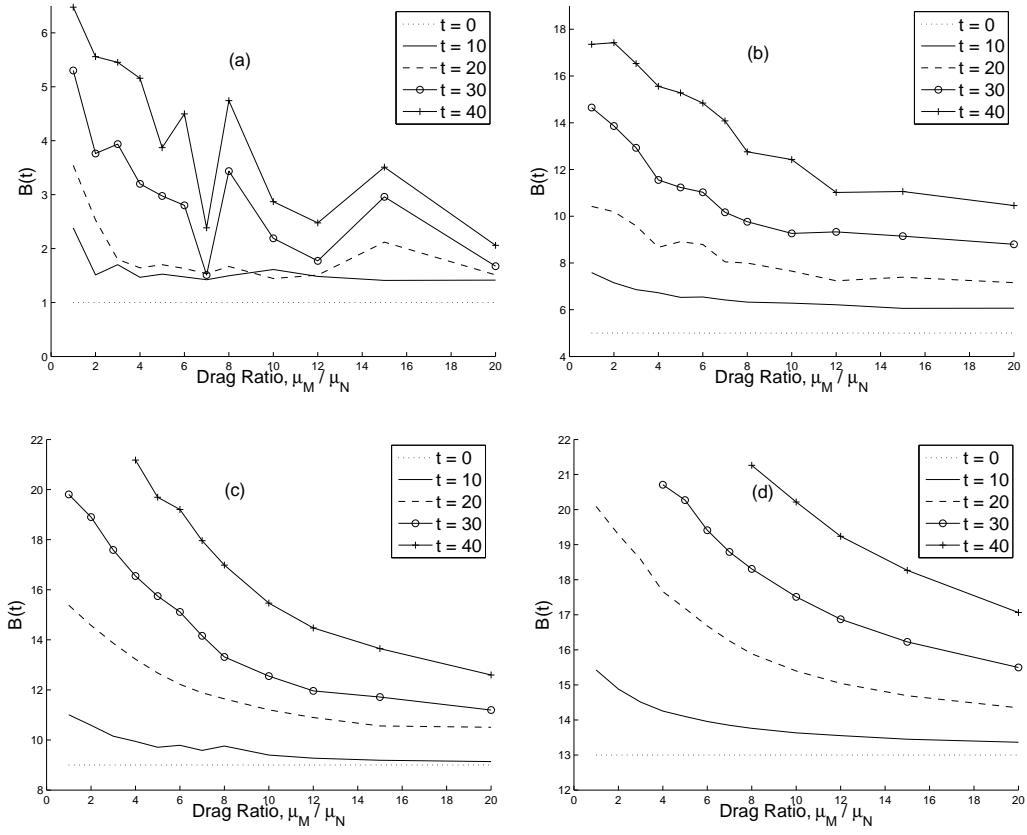
Figure 5.6: Series of plots showing how B(t) , the position of the lowest cell in the mutant patch in the cell-centre model varies with the drag ratio, \mu_M / \mu_N , with position plotted after t = 0, 10, 20, 30, 40 hours. Plots are for different initial positions of the circular mutant patch of initial radius 2 and azimuthal position x = 0 and y = A_0 , with (a) A_0 = 3 , (b) A_0 = 7 , (c) A_0 = 11 , (d) A_0 = 15 .
