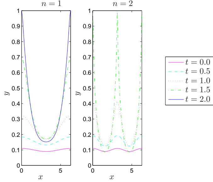
Figure 2.13: Series of plots showing showing how the boundary y = \chi(x, t) changes over time and how this evolution depends on which spatial modes are being excited. The simulations suggest that if the type 2 cells are 10 times more viscous than the type 1 cells then at long times they may migrate downwards, towards the crypt base. The plots have initial conditions of \chi_0 = 0.1 + 0.005 \cos(nx/\beta) , where n = 1 (left) and n = 2 (right). Parameter values: D = 0.1 , k = 3 , \lambda_1 = 1.5 , \lambda_2 = 0 and \beta = 1 .
