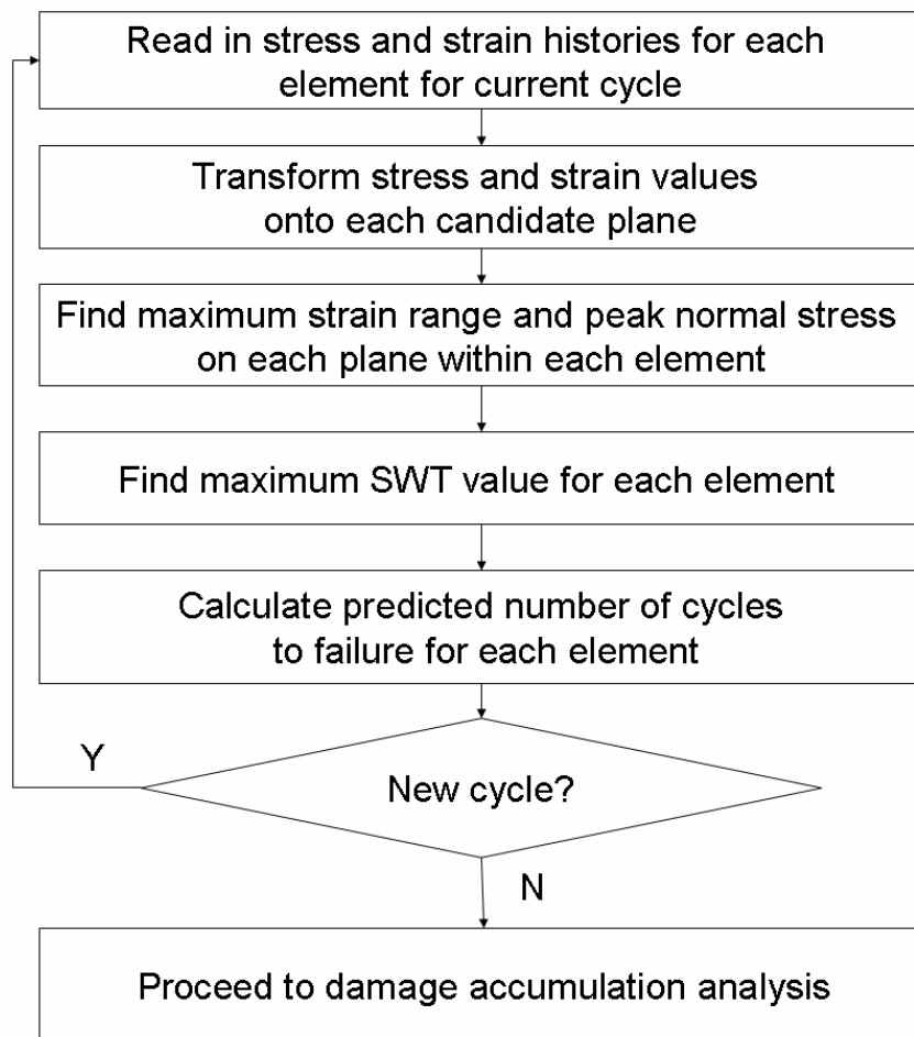
Figure 3.7. Flow chart showing the process for calculating the critical plane SWT value for wear simulations.
