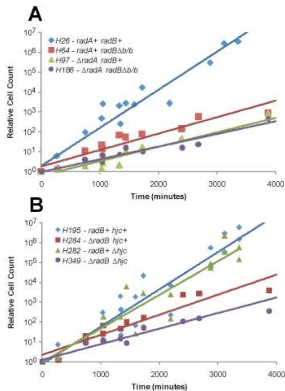
Figure 3.26 Growth rates in strains deleted for genes that encode proteins shown to interact with RadB in vitro . A Growth rates of H26 ( radA+ radB+ ), H64 ( radA+ radBΔb/b ), H97 ( ΔradA radB+ ) and H186 ( ΔradA radBΔb/b ) to determine the effect of ΔradA . B Growth rates of H195 ( hjc+ radB+ ), H284 ( hjc+ ΔradB ), H282 ( Δhjc radB+ ) and H349 ( Δhjc ΔradB ), to determine the effect of Δhjc . Relative cell count is calculated as a proportion of the cells present at time = 0 minutes. Data points are consolidated from three trials.
