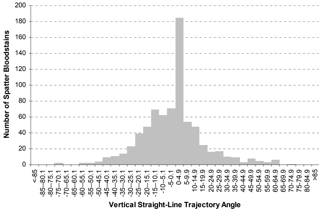
Figure 8-12 - An example of the raw count data generated during the characterisation of a collection of spatter bloodstains based on the vertical angle of the constructed straight-line trajectory approximations.
