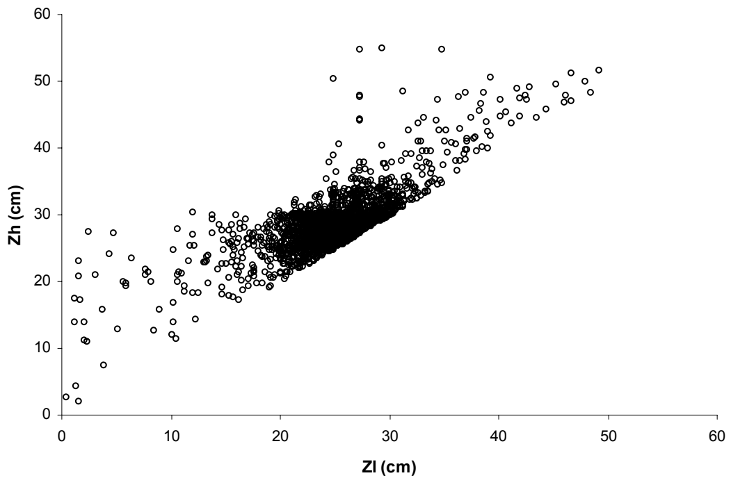
Figure 9-10 - A scatter plot of the p_{z1} and p_{zh} trajectory intersection data generated during the analysis of the 0-5 cm 3D data quality sample of pattern ES-A.
