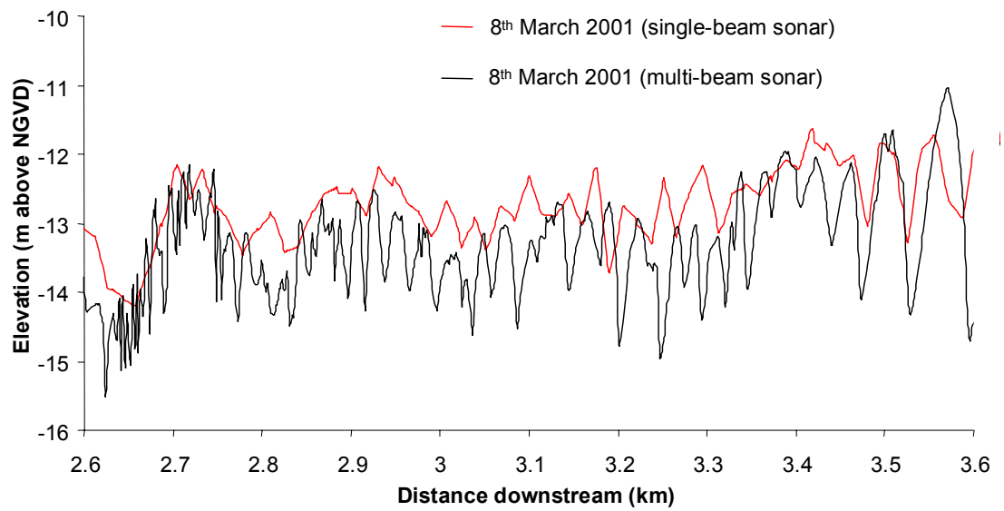
Figure 7.16 Area D of Figure 7.11 enlarged to compare dune characteristics obtained from multi-beam sonar with dune characteristics obtained from single beam sonar. Both surveys were undertaken on the 8 th March 2001 and are extracted from TIN topographic surfaces at regular 1.5 m intervals.
