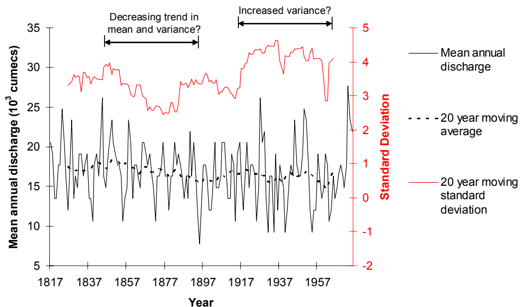
Figure 4.20 Trends in mean annual discharge in the period 1817-1975 based on data from Winkley (1977). Data is for calendar year at Vicksburg. See text for further description.
