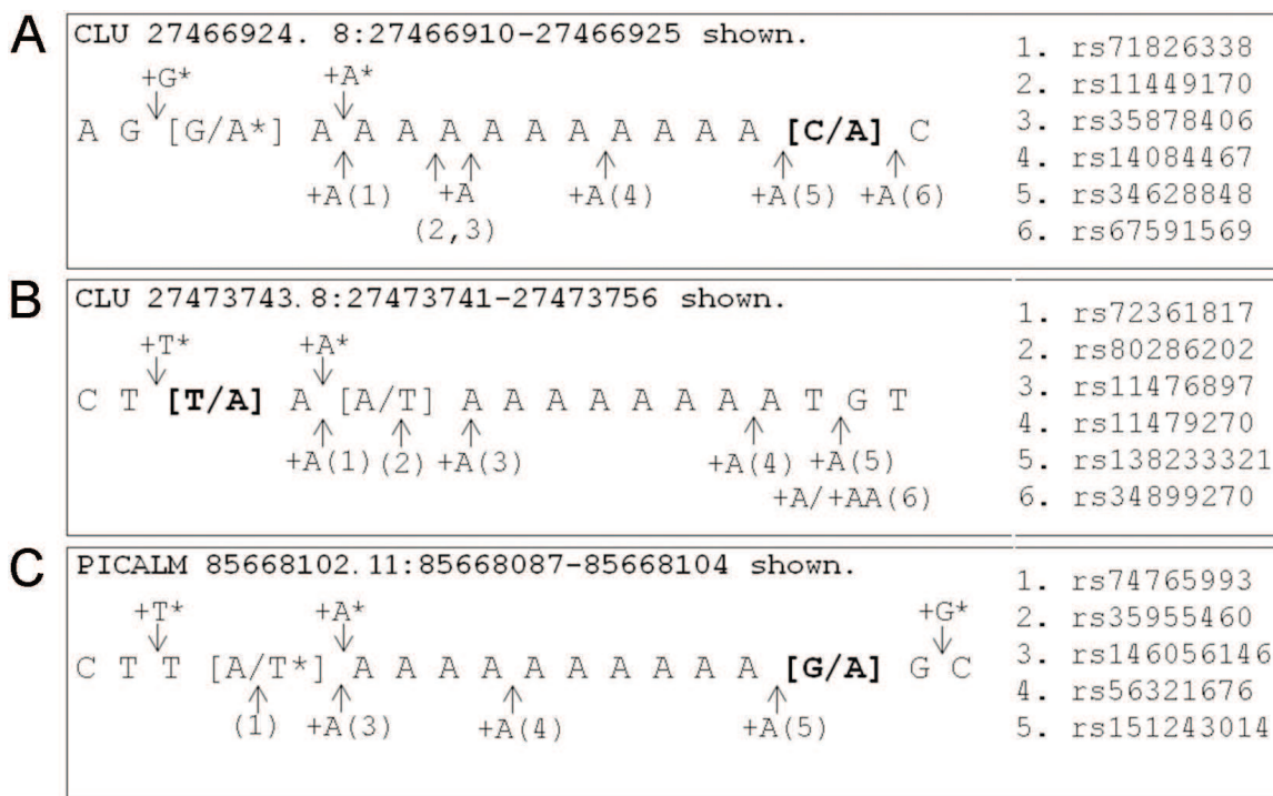
Figure 1. Sequence context of spurious SNPs called next to mononucleotide repeats, which failed validation by Sanger sequencing. The SNP shown in bold is the variant Sanger sequencing was designed to validate. Variants shown below the sequence are all present in dbSNP. A: False C/A variant call within CLU at position 8:27466924 (8:27466910-27466925 shown). B: Spurious T/A SNP call in CLU at 8:27473743 (8:27473741-27473756 shown). C: False positive SNP call at position 11:85668102 within PICALM (11:85668090-85668104 shown). *Other variants called by CRISP.
