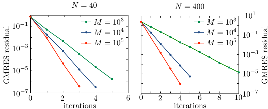
Fig. 5.3: Convergence of GMRES iterations for the problem \mathbf{DF}(\mathbf{U})\mathbf{V} = -\mathbf{F}(\mathbf{U}) , where \mathbf{U} is a macroscopic front and \mathbf{DF}(\mathbf{U}) = \mathbf{I} - \mathbf{D}\Phi_T^M(\mathbf{U}) , for different numbers of agents N and numbers of realizations M . Jacobian actions are computed with weighted lifting and \varepsilon = 10^{-5} .
