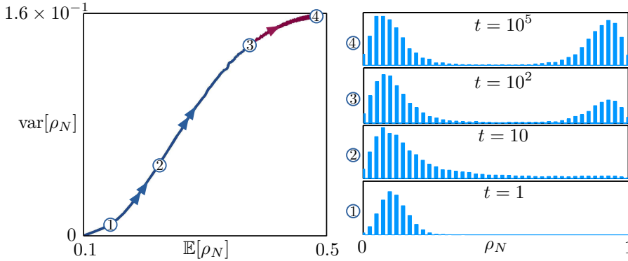
Fig. 2.3: Expectation and variance of the average agents’ choice \rho_N(t) = \sum_n u_n(t) for the lock-in model with N = 40 agents (see also the animation slaving.avi ). Left: we initialise M = 10^4 realizations from u_{0n} = 0.1 for all n ; the evolution on the (\mathbb{E}[\rho_N], \text{var}[\rho_N]) -plane is plotted with a blue line for the first 10^2 iterations and in magenta for the following iterations, until t = 10^5 . Right: distributions of \rho_N at various times. After a short transient, the evolution takes place on a slow manifold. Parameters: \bar{\mu} = 0 , \Delta\mu = 0 , \alpha = 0 , \bar{\xi} = 0.235 , \bar{\nu} = 0.3 , \bar{\zeta} = 0.03 , \beta = 8 .
