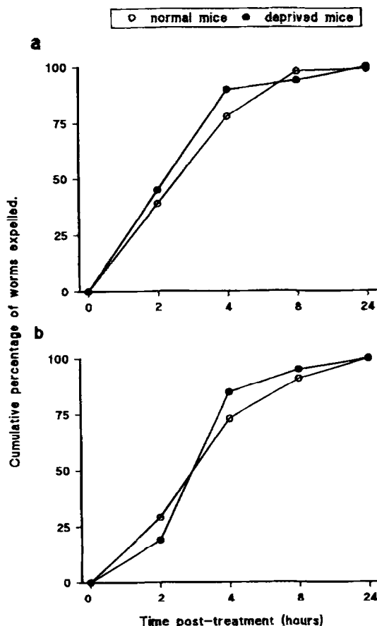
Fig. 1. Cumulative percentage of worms recovered in faeces of Heligmosomoides polygyrus -infected normal and T-cell-depleted mice following treatment with (a) pyrantel pamoate or (b) levamisole. Faecal samples were collected prior to treatment (0) and 2, 4, 8 and 24 h after administration of the drug.
