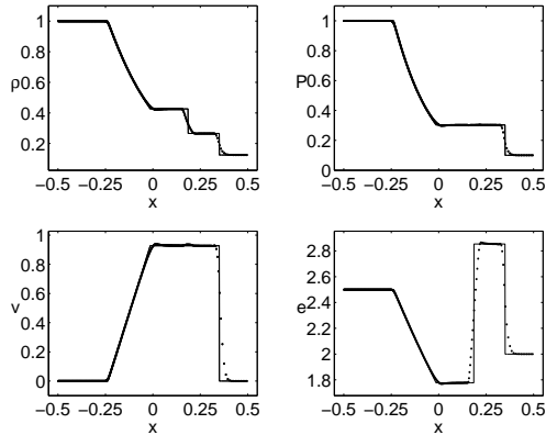
Fig. 2. Shock tube simulation ( t=0.2 ) using linearly complete MLS shape functions.
