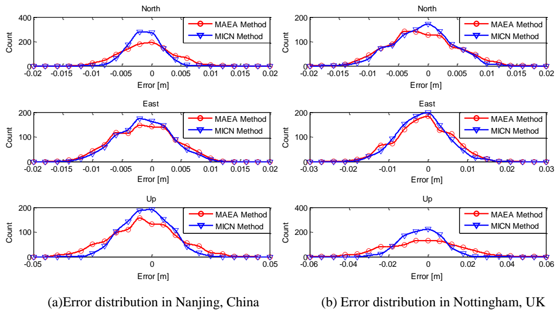
Figure 13. Positioning error distribution for East-West blockage.
