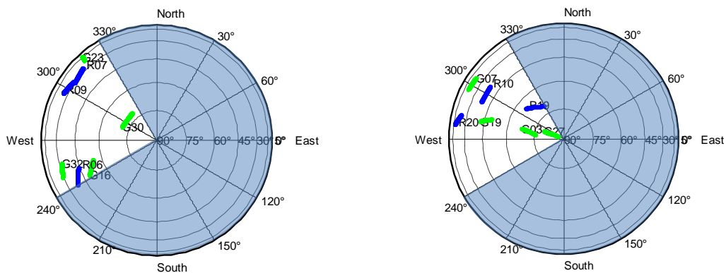
(a) Satellite sky plot in Nanjing, China (b) Satellite sky plot in Nottingham, UK
