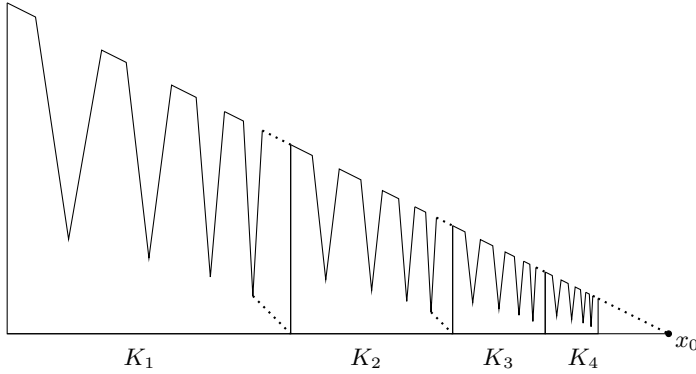
Fig. 2. A compact set X , where R(X) admits exactly one R-point (the point x_0 ), but no points of continuity
