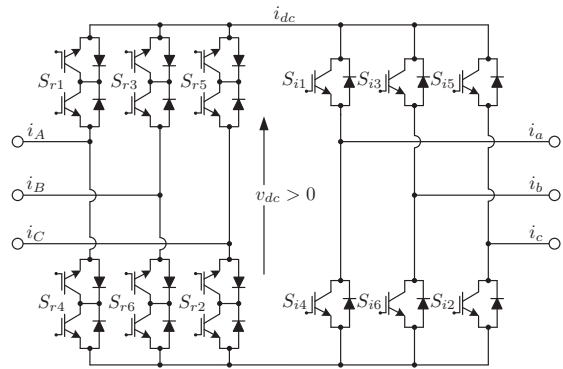
Fig. 4. Conventional indirect matrix converter (common collector).
