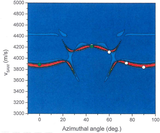
FIG. 4: Simulation of the azimuthal angle dependence of the SAW velocity for the c-GaN layer on GaAs using the set of elastic constants determined in this work (see Table I). The circles represent SAW velocities at different azimuthal angles determined by HRBS measurements.
