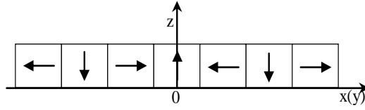
Fig.6. One dimension quasi-Halbach PM array.
