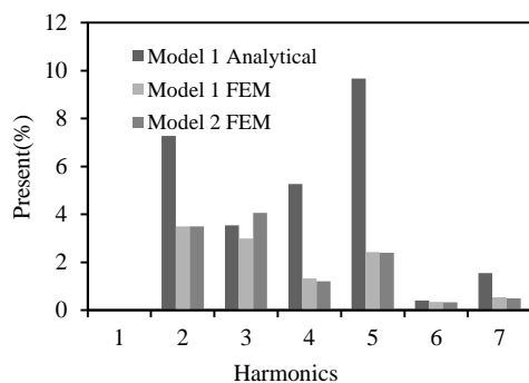
Fig.10. Comparison of the harmonics in B_{zav} (airgap=2mm).
