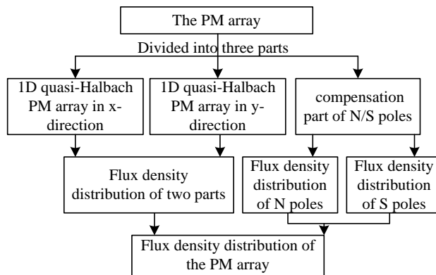
Fig.5. Overall diagram of the analytical model.
