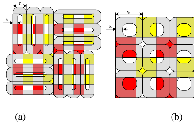
Fig.13. Winding topology of (a) Compter [22], (b) Kou [23].
