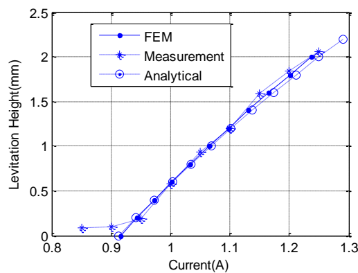
Fig.18. Relationship between levitation height and current.
