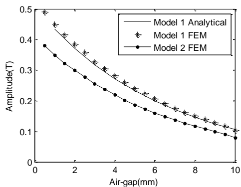
Fig.9. Amplitude of fundamental wave in B_{zav} .
