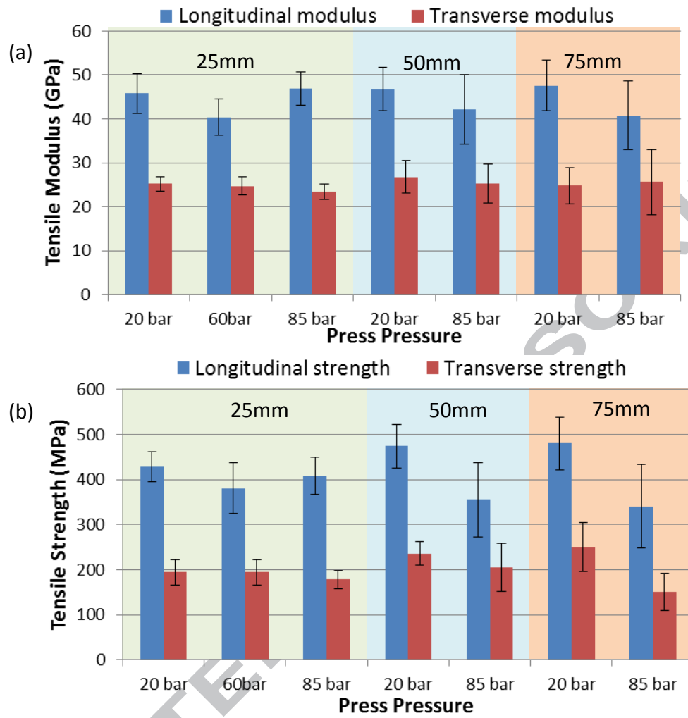
Figure 13: Tensile modulus (a) and strength (b) of different fibre length DFC compounds with 50% mould coverage and 50% Vf, varying the moulding pressure.
