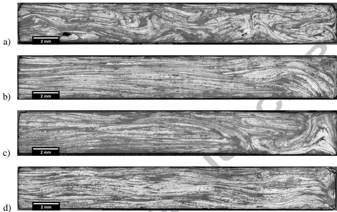
Figure 8: Micrographs (5x magnification) of the right hand edge, end of flow, for 40% (a), 60% (b), 80% (c) and 100% (d) mould coverages. All images are parallel to the flow direction
