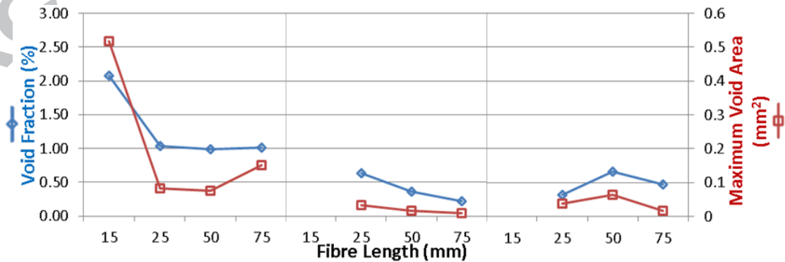
Figure 14: Void content for varying fibre lengths for 100% charge coverage at 85 bar (left), 50% charge coverage at 85 bar (middle), and 50% charge coverage at 20 bar (right)
