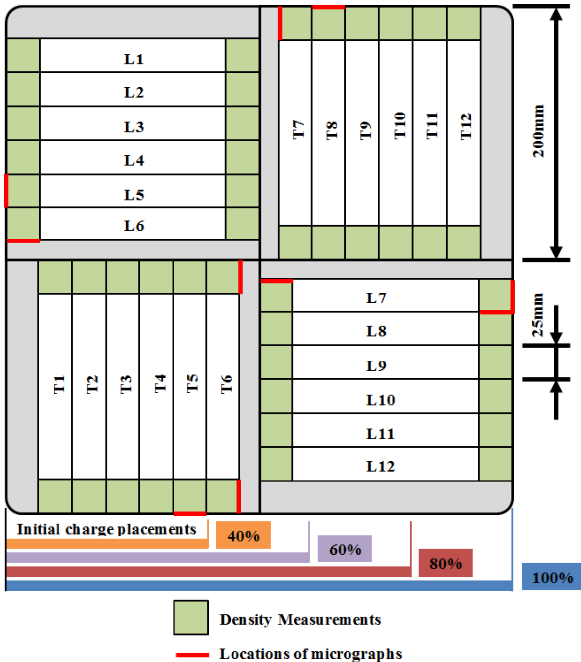
Figure 3: Initial charge position and cutting plan for the 405mm x 405mm plaques. Locations for tensile coupons, density measurements and micrograph shown.
