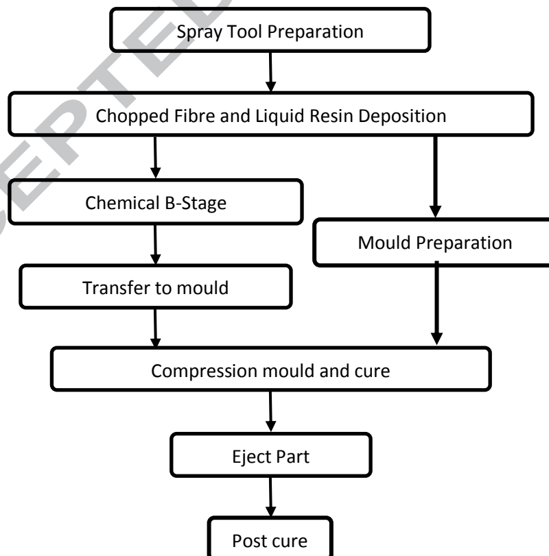
Figure 2: DFC flow chart
