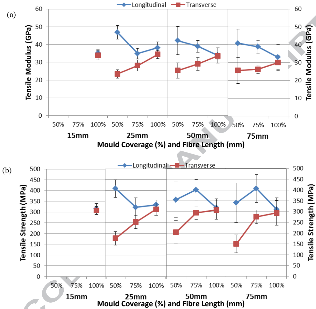
Figure 10: Effect of fibre length on tensile modulus (a) and tensile strength (b) for DFC compounds with 50%, 75% and 100% mould coverages (50% Vf).
