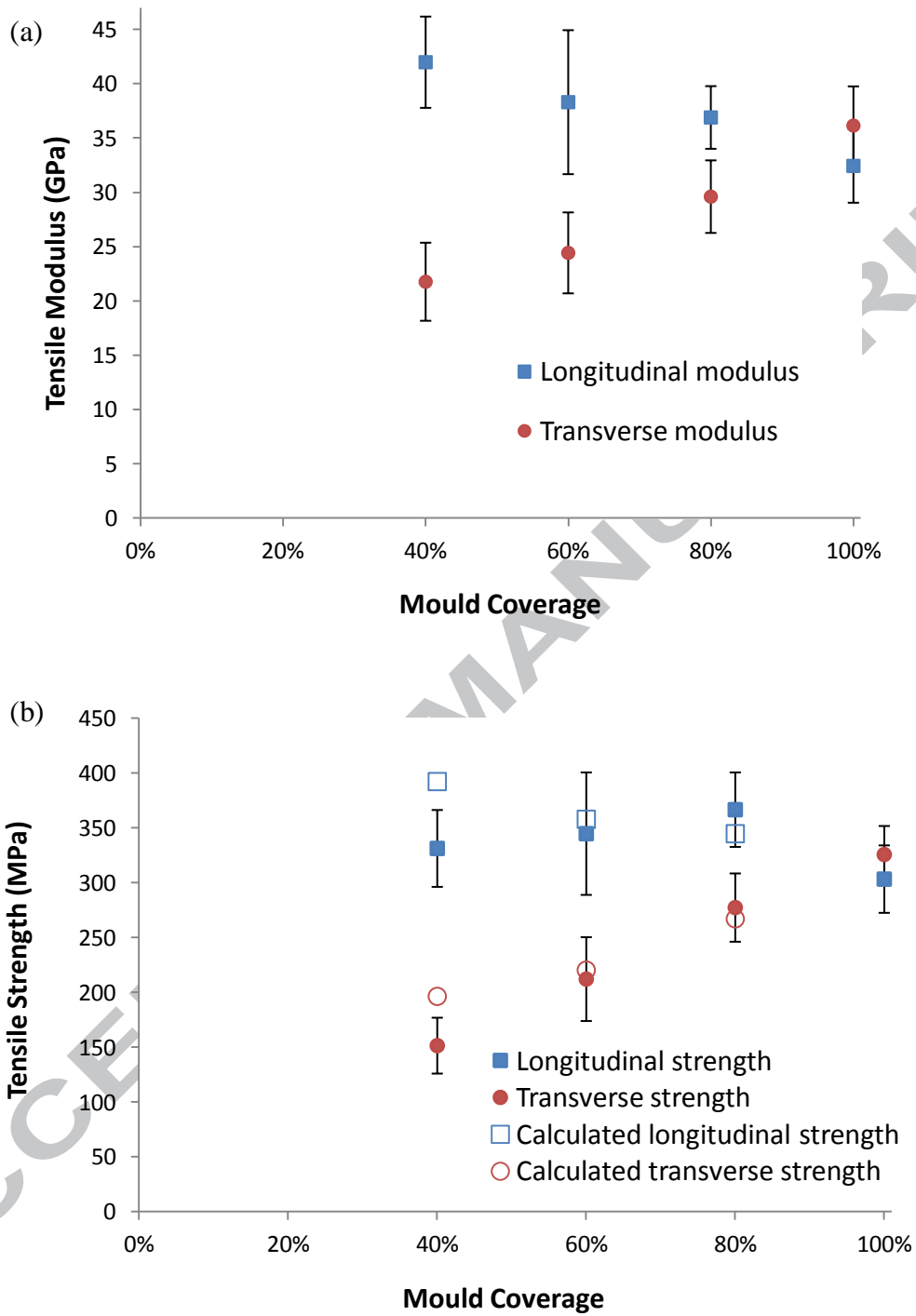
Figure 7: Tensile modulus (a) and strength (b) of DFC plaques. (25mm fibre length, 45% V_f )
