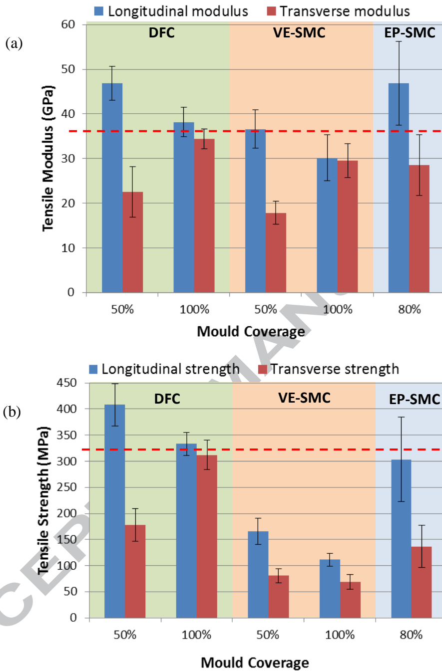
Figure 4: Tensile modulus (a) and tensile strength (b) as a function of mould coverage. All materials moulded at 85 bar. The red dotted line represents the average of the longitudinal and transverse properties of the 100% coverage DFC material.
