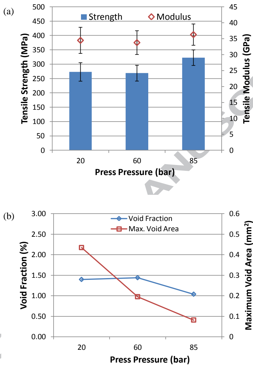
Figure 12: The effect of mould pressure on tensile properties (a) and void content (b) for 100% net-shaped compounds
