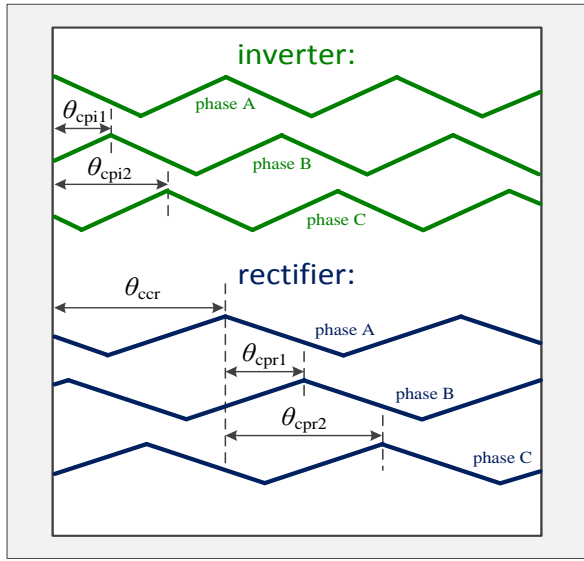
Fig. 2. Definition of carrier phase shifts
