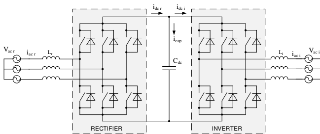
Fig. 1. Diagram of two-level back-to-back converter
