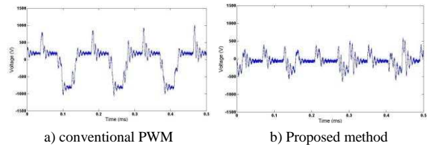
Fig.13. Comparison of common-mode voltages
