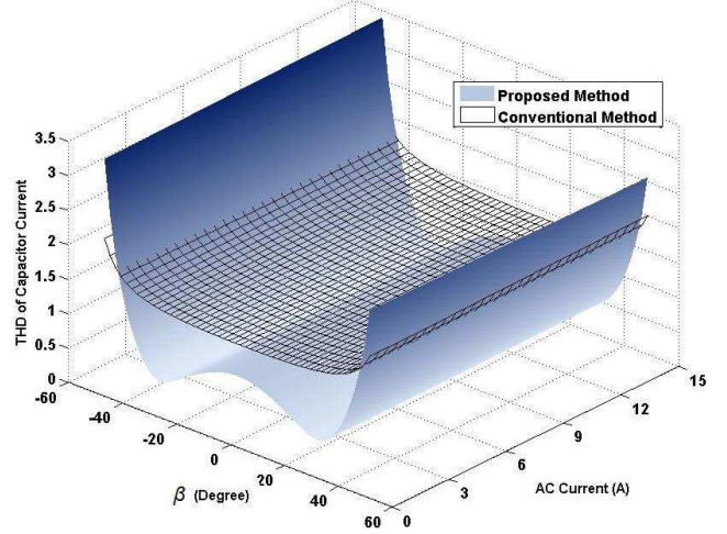
Fig.11. THD assessment under different I_{ac} and \beta .
