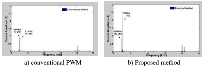
Fig.14. Comparison of AC current harmonic spectrum for rectifier
