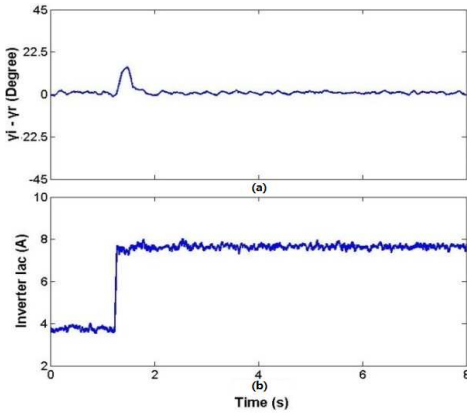
Fig.10. Harmonics phase difference in response to change in operation conditions (Inverter power factor is fixed at 0.92, and the ac current amplitude steps from 3.9A to 7.8A)
