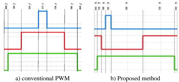
Fig.12. Effect of inter-leg carrier phase shift on the PWM pattern
