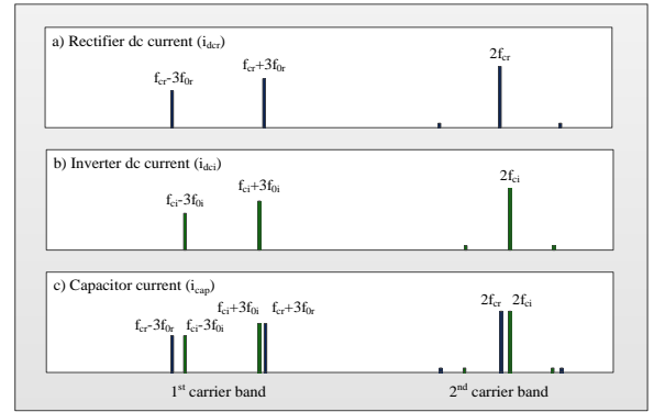
Fig. 3. Original DC-link current spectrum with conventional SPWM
