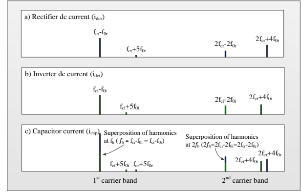
Fig. 5. DC-link current spectrum following Step 2.
