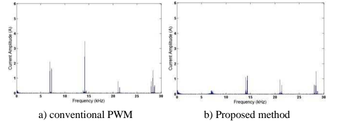
Fig. 9. DC-link capacitor current spectra
