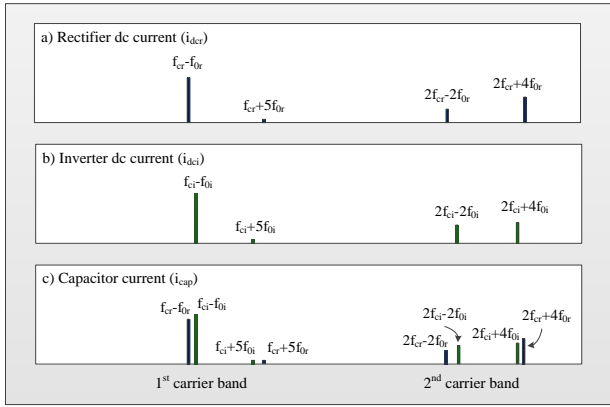
Fig. 4. DC-link current spectrum following Step 1.
