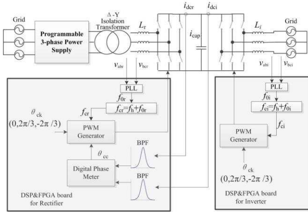
Fig. 7. Test rig control for the experimental verification
