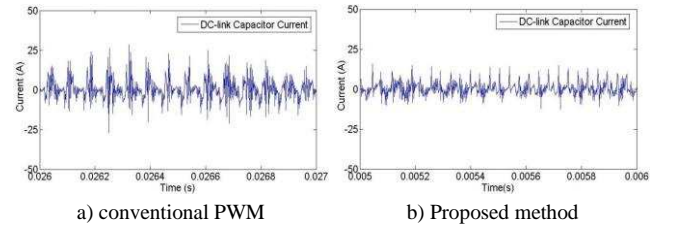
Fig. 8. DC-link capacitor current waveform
