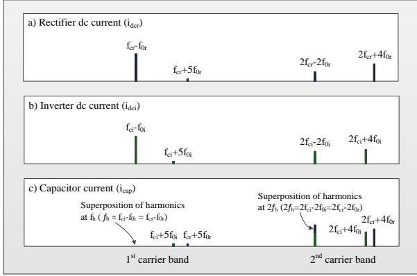
Fig. 6. DC-link current spectrum as a result of Step 3.
