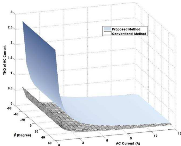
Fig. 15. THD comparison for the ac-side current
