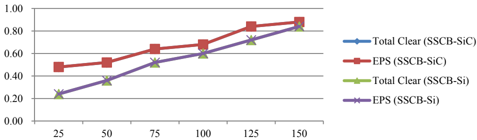
Fig. 14: Comparison of total clear time and EPS trip time (ms) with SiC MOSFET and Si IGBT.
