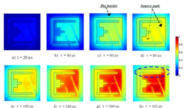
Fig. 6. Thermal maps of the chip surface corresponding to the short-circuit pulses of Fig 5. The scale is normalized to the maximum measurable temperature (ca. 500 ^{\circ}\text{C} ).
