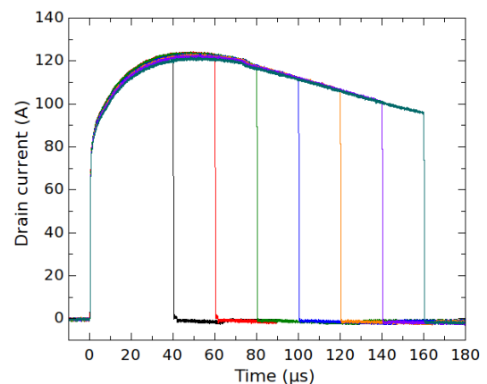
Fig. 5. Short-circuit current waveforms with V_{DS} = 100\text{V} ; and T_{CASE} = 20^{\circ}\text{C} .
