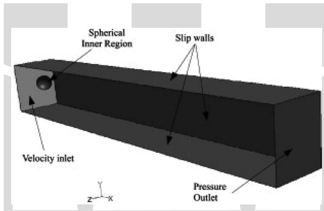
Fig. 6. Computational domain and boundaries for free-flight simulation of debris [13]
