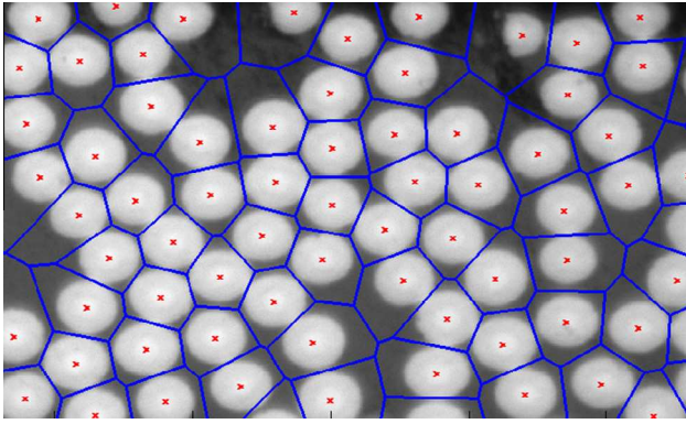
Fig. 5. Section of a micrograph of a carbon fibre bundle overlaid with polygons as a result of a Voronoi cell tessellation. (For interpretation of the references to colour in this figure legend, the reader is referred to the web version of this article.)
