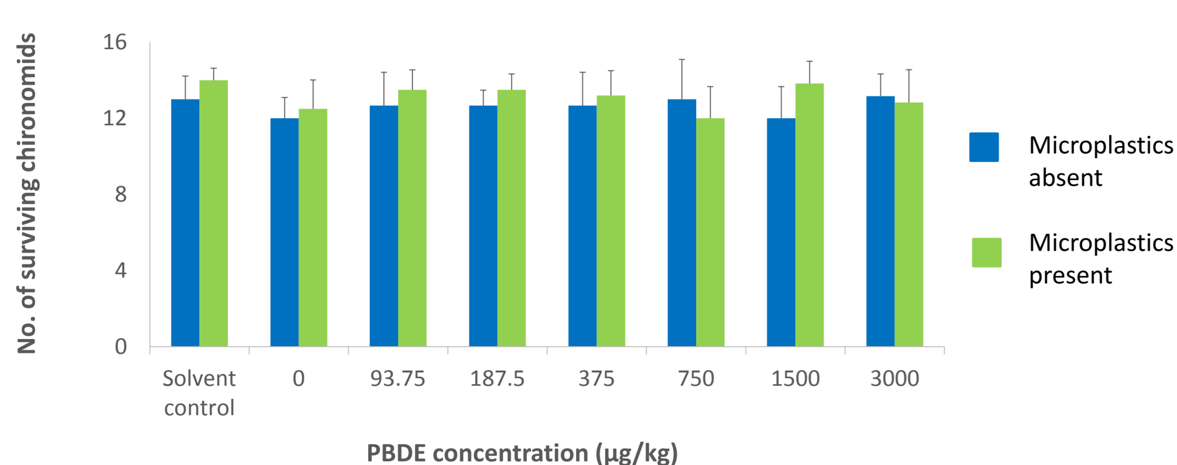
Fig 2. Survival of chironomids after 96 hours exposure to PBDEs in the presence and absence of nylon microparticles.
