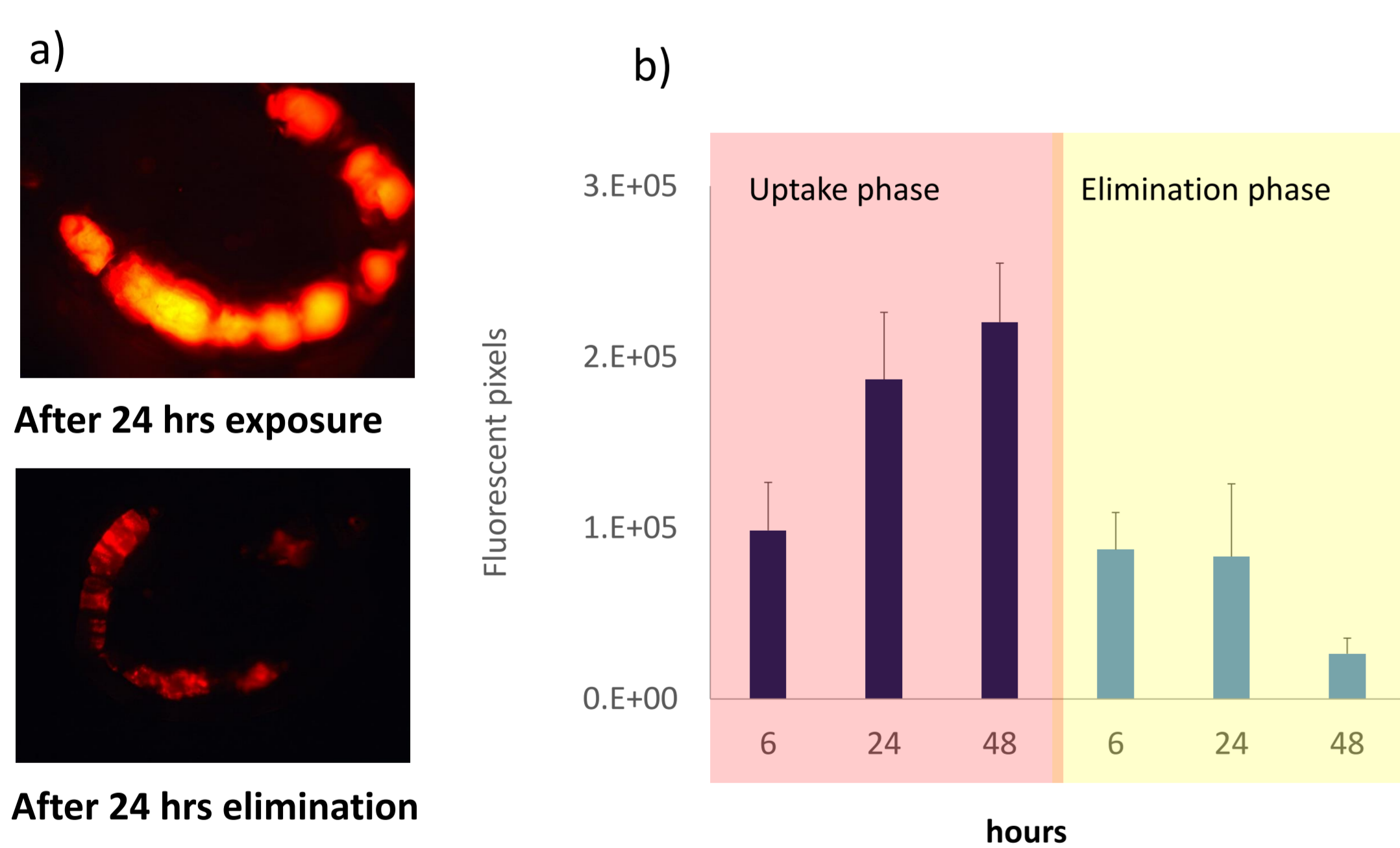
Fig 1: (a) Images (left) of chironomid taken under a fluorescence microscope after 24 hours exposure (top) to 1% nylon in sand and following 24 hours elimination (bottom) in clean sand. (b) The uptake and elimination over the two 48 hour periods
