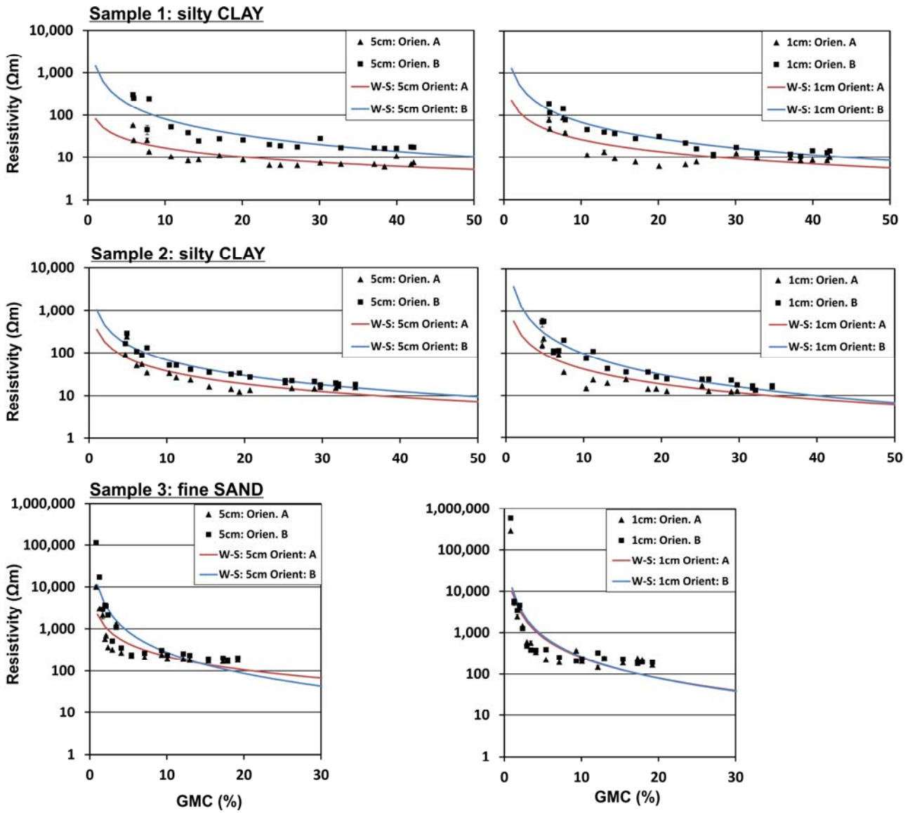
Figure 5. Electrical resistivity – soil moisture content relationship of earthflow deposits of the Hollin Hill landslide system. Presented are the associated Waxman-Smits models for each of the electrical measurement orientations.
