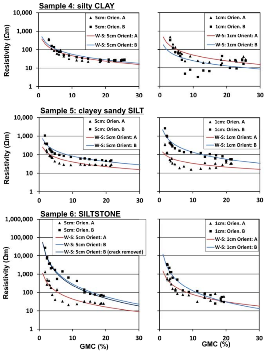
Figure 6. Electrical resistivity – soil moisture content relationship of slump deposits and in-situ material of the Hollin Hill landslide system. Presented are the associated Waxman-Smits models for each of the electrical measurement orientations.
