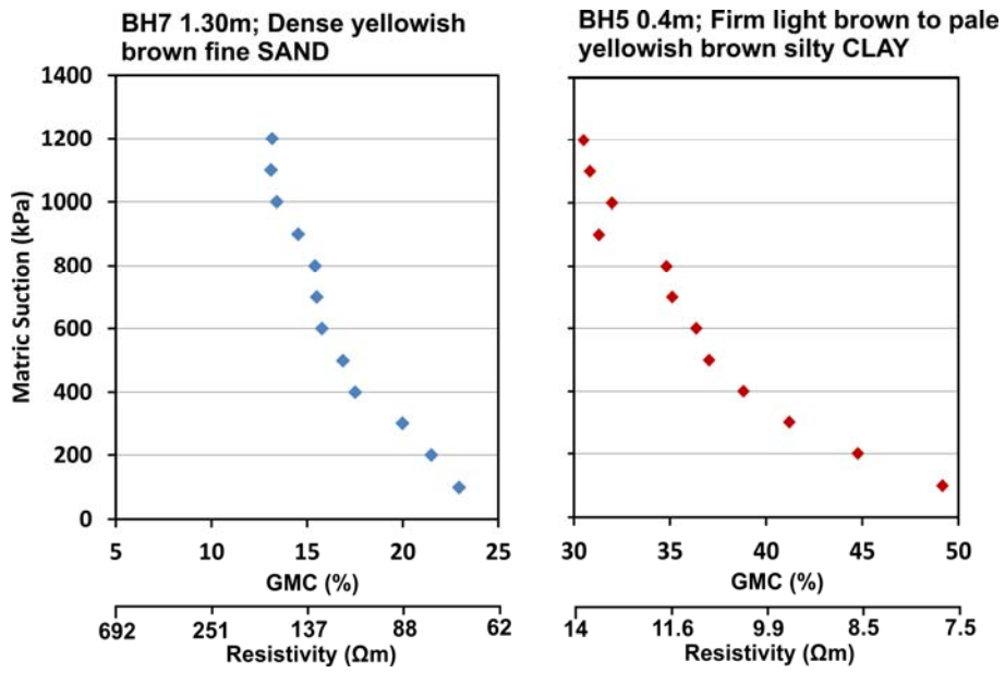
Figure 7. Soil moisture retention curve of two earthflow samples, extracted from Hollin Hill soil cores. a) (left) BH7, 1.30 m, and b) (right) BH5, 0.40 m. NB, non-linear electrical resistivity axes.
