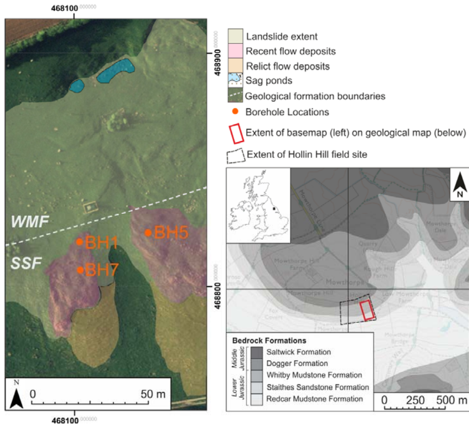
Figure 1. Geological maps of the field site, showing major lithological and geomorphological divisions and borehole locations.
