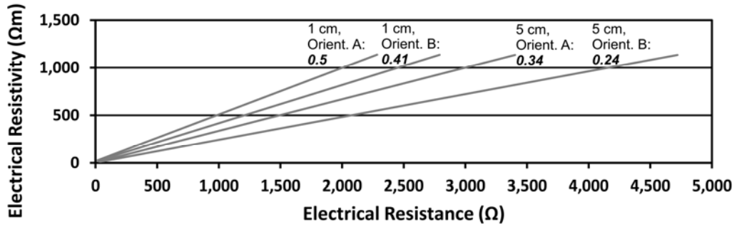
Figure 4. Relationship between saline solution electrical resistivity ( \rho_a ), measured electrical resistance ( R ) and calculated geometric factor ( k ) for each electrode array size and measurement orientation.
