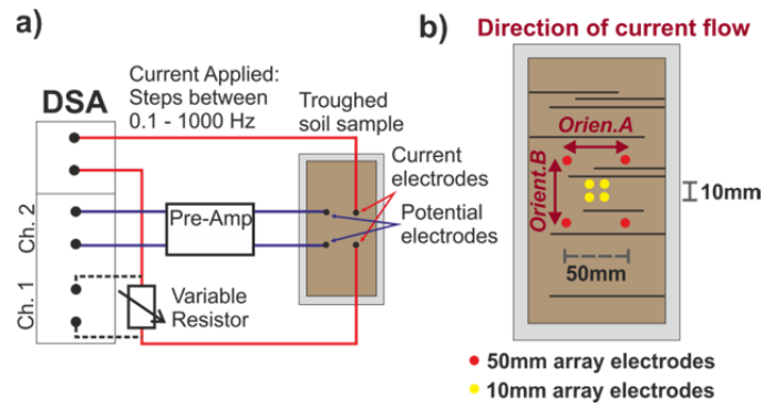
Figure 3. a) (left) Electrical circuit diagram of Digital Signal Analyser circuit board and pre-amplifier experimental setup (adapted from Ntarlagiannis et al., 2005) b) (right) Diagram of sample trough along with electrode array locations, measurement dimensions and current flow directions.
