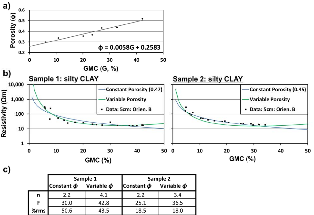
Figure 8. Comparison between Waxman-Smit models between porosity-constant and porosity-variable models.
