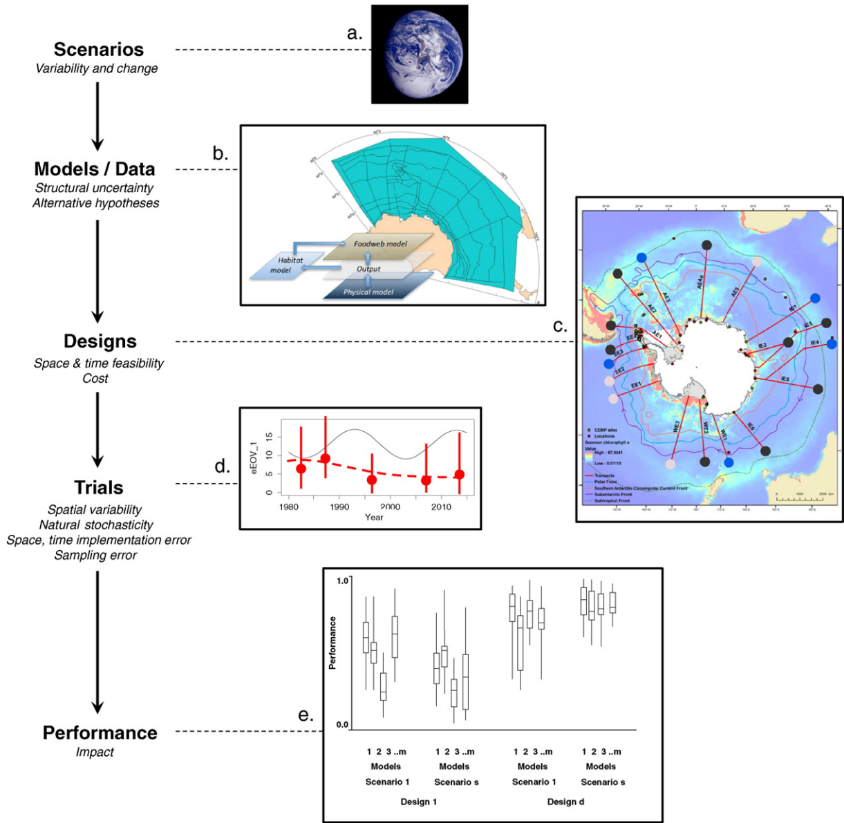
Fig. 3. Important steps in the process for evaluating candidate eEOVs using case studies and model simulations (see text for explanation). a. Scenarios derived from hypothesised or modelled time-series of global or regional physical forcings. b. Models/data used to generate time-series of ecosystem properties, represented here by a schematic of a coupled end-to-end ecosystem model for the Indian Sector of the Southern Ocean, based on physical, habitat and food web sub-models. c. Alternative sampling designs in space and time for measuring the candidate eEOVs and tested against the criteria in Table 4 (Fig. 5 is reproduced here showing a possible design based on current field capability). d. Trials of a design used to generate a time-series of observed eEOVs using the proposed sampling design (circles with error bars and a fitted dashed line) to compare with the actual time-series of the quantities in the model (solid line). e. The performance of a design, with the figure showing the performance (box plots illustrate variability in performance across many randomised trials) of 2 field designs for 2 plausible future scenarios and based on 4 different plausible models of the ecosystem.
