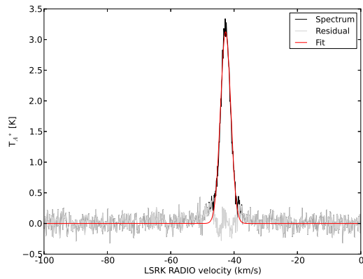
(c) \text{HCO}^+
