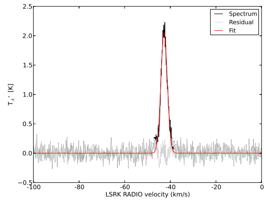
(b) HNC
