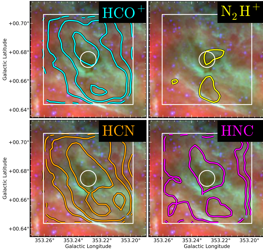
Figure 6. MALT90 images of the ATLASGAL continuum source G353.229+00.675. The color images are GLIMPSE/MIPSGAL 3-colour images with blue = 3.6 \mu\text{m} , green = 8.0 \mu\text{m} , and red = 24 \mu\text{m} . The contours represent integrated intensity molecular line emission from MALT90, with \text{HCO}^+ (1-0) in cyan (upper left), \text{N}_2\text{H}^+ (1-0) in yellow (upper right), \text{HCN} (1-0) in orange (lower left), and \text{HNC} (1-0) in pink (lower right). Contour levels are drawn at signal-to-noise levels of 1.5, 3, 7, 11, and 17. This is an example of a source with weak or absent \text{N}_2\text{H}^+ emission, but strong \text{HCO}^+ , \text{HCN} , and \text{HNC} emission. Since the maps were taken simultaneously, the variations in intensity are real and not due to calibration errors. The circle represents the Mopra FWHM beam.
