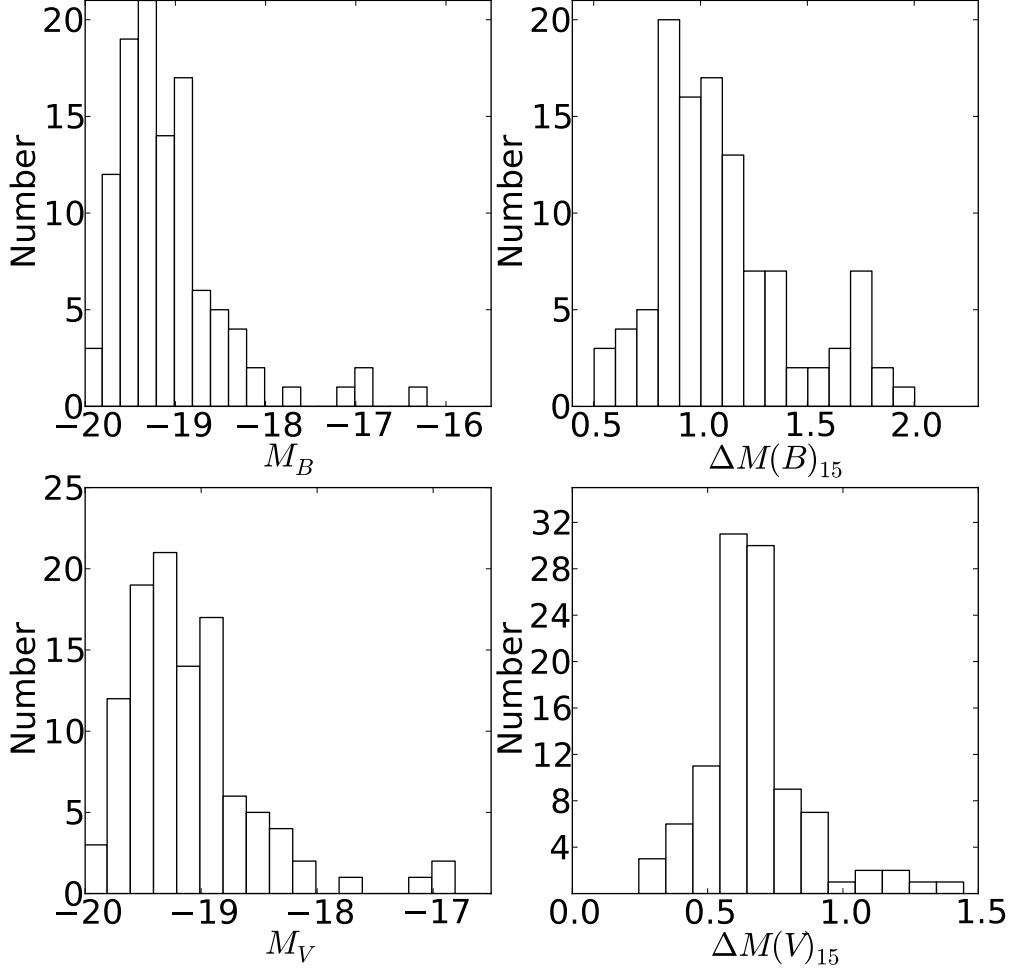
Figure 7. Top: B -band luminosity distribution, corrected for host galaxy extinction. The bin sizes are 0.15 and 0.1 mag for the M_B and \Delta m_{15}(B) plots respectively. Bottom: V -band luminosity distribution, corrected for host galaxy extinction. The bin sizes are 0.15 and 0.1 mag for the M_V and \Delta m_{15}(V) plots respectively.
