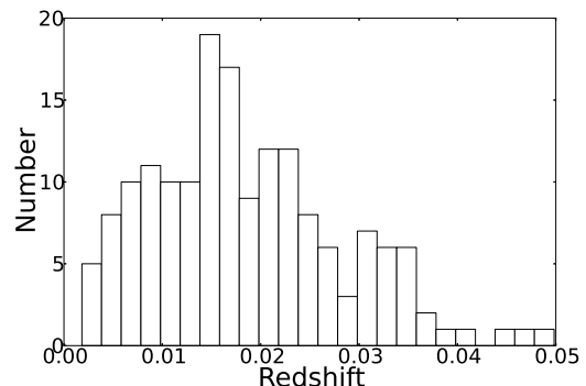
Figure 1. Redshift distribution of the SNe Ia used in this paper. The bin sizes are z=0.002 .
