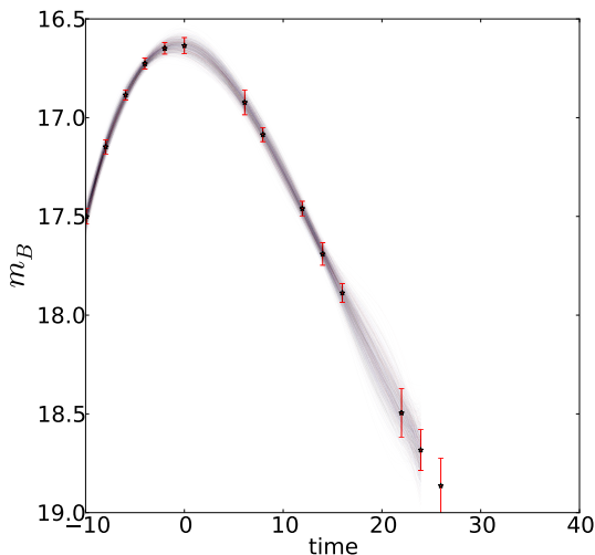
Figure 2. An example of the fitting procedure, the B -band light curve of SN 2000dn. The red points are the photometry and the shaded area is the 1000 LCs derived from these photometry points, as explained in section 2.1.
