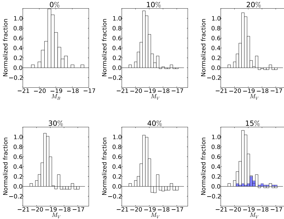
Figure 13. The V-band LD for SNe Ia from passive galaxies normalized, scaled and subtracted from the LD of SNe Ia from S-F galaxies. The factor by which the SNe Ia from passive galaxies has been normalized is presented on the top of each plot. The blue bars in the bottom right panel are the LD of SNe Ia from passive galaxies scaled to 15% of those from active galaxies.
