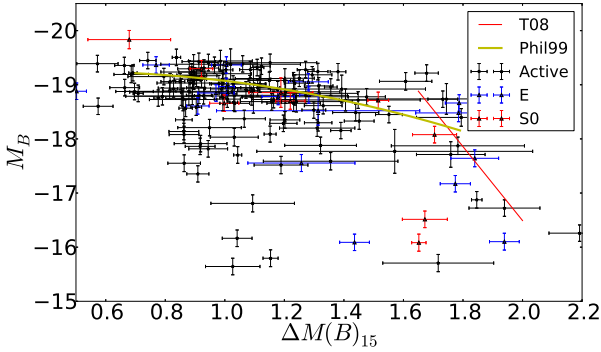
Figure 4. The B -band WLR before reddening correction. The black points are SNe from S-F galaxies, the blue points are SNe from E galaxies, and the red points are SNe Ia from S0 galaxies. The yellow line is the WLR given in Phillips et al. (1999), and the red line is the relation given for the subluminous tail from Taubenberger et al. (2008).
