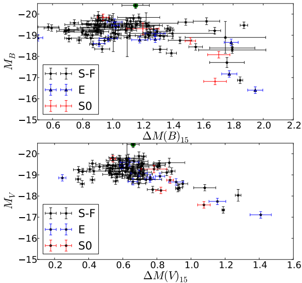
Figure 9. The WLR corrected for host galaxy extinction. The black points are SNe from S-F galaxies, the blue are points are SNe from elliptical galaxies and the red points are SNe Ia from S0 galaxies. The green point is SN2003cg. Top: B-band Bottom: V-band
