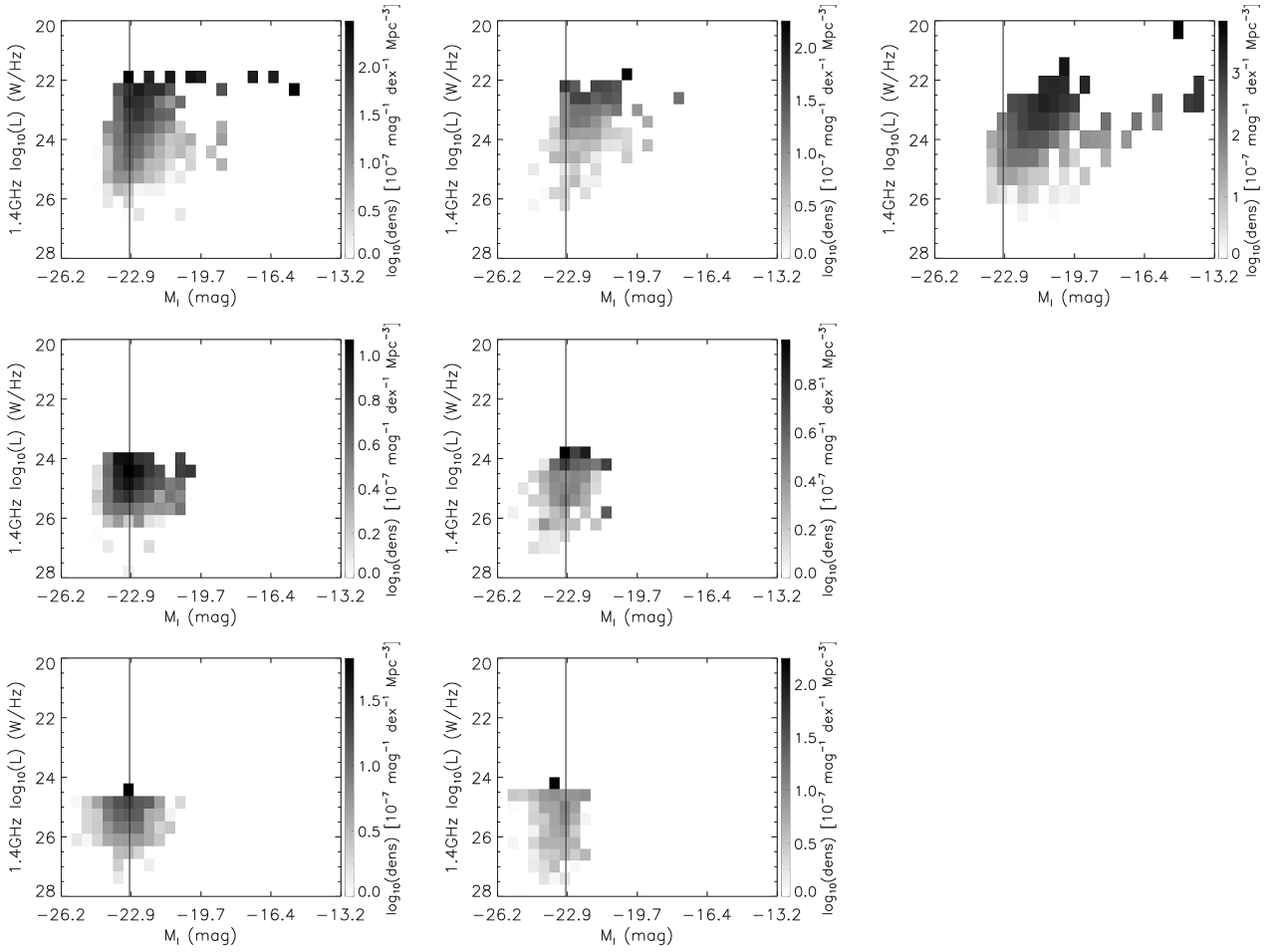
Figure 6. The bivariate luminosity distribution for LERGs (left column), HERGs (middle column) and star forming radio galaxies (right column). The rows are for the different redshift bins: top row : 0.005 < z < 0.30 ; middle row : 0.30 < z < 0.50 ; and bottom row : 0.5 < z < 0.75 . Only the lowest redshift bin is shown for the star-forming radio galaxies since there are no objects with this classification in higher redshift bins. The flux-density and apparent magnitude selection limits correspond to progressively brighter radio and optical luminosity limits with increasing redshift. The absolute magnitude limit applied when analysing the redshift evolution of the radio luminosity function is shown as the vertical line. This corresponds to the absolute magnitude limit at the high-redshift edge of the highest redshift bin.
