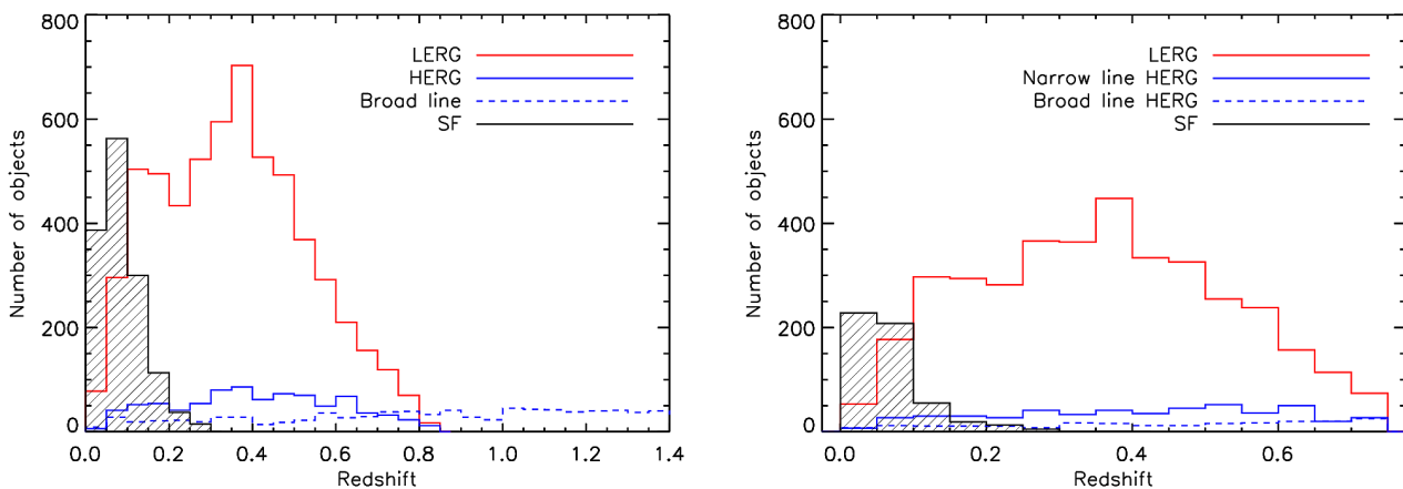
Figure 2. Left panel: The redshift distribution of all radio galaxies with reliable spectroscopic redshifts. The redshift distributions for star-forming galaxies, LERGs and HERGs are shown separately. Above z \sim 0.8 the sample is dominated by broad-line AGN. Right panel: The n(z) of the sample used to construct luminosity functions in this paper after selecting objects with 0.005 < z < 0.75 and S_{1.4\text{GHz}} > 2.8 mJy.
