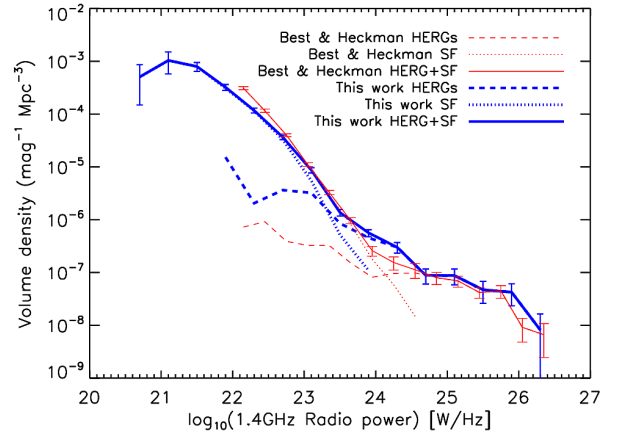
Figure 8. Top panel: the radio luminosity function of star forming radio galaxies (blue dotted line), HERGs (blue dashed line) and their sum (blue solid line) in our sample and those from Best & Heckman (2012) (red dotted, red dashed and red solid lines, respectively). The bottom panel is the same as the top panel but with the broad line AGN removed from our HERG sample.
