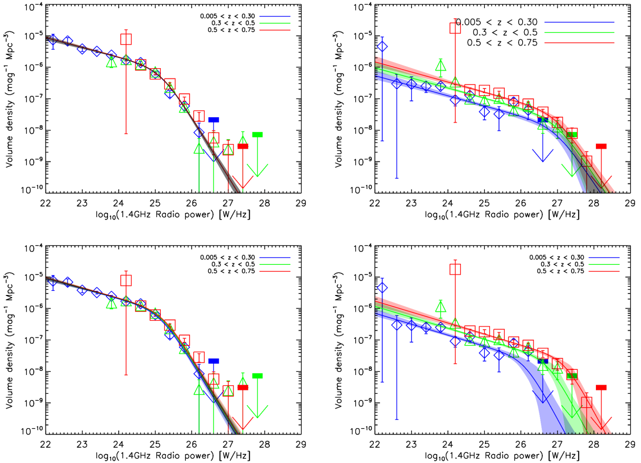
Figure 10. The radio luminosity function for LERGs ( left column ) and HERGs ( right column ) separated into three redshift bins: 0.005 < z < 0.30 ( blue ); 0.30 < z < 0.50 ( green ); 0.5 < z < 0.75 ( red ). The top row shows the fit to the data ( solid lines ) assuming pure density evolution and the bottom row show the fit to the data assuming pure luminosity evolution.
