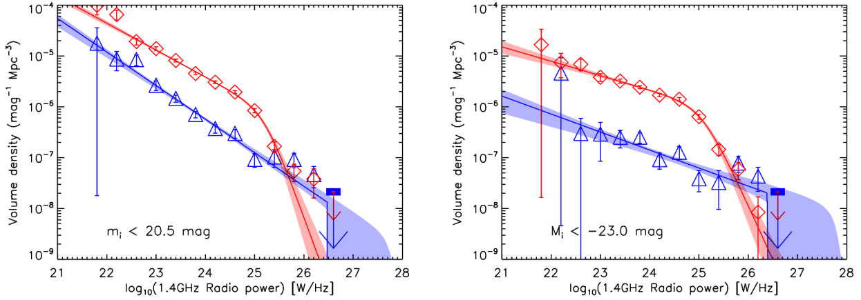
Figure 9. The radio luminosity function of AGN in our 0.005 < z < 0.3 redshift bin separated into LERGs ( red diamonds and solid line ) and HERGs ( blue triangles and solid line ). Left panel : integrated over i < 20.5 and right panel : galaxies with M_i < -23 only. Over-plotted are double power law fits to the data ( solid lines ).
