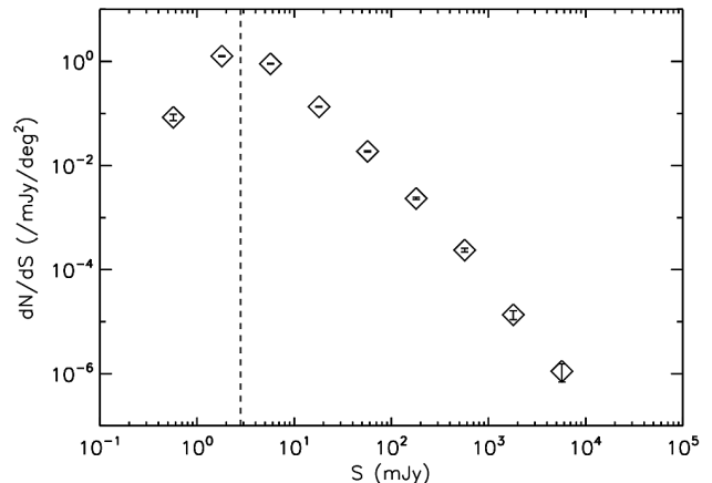
Figure 1. Number of objects per interval of 1.4 GHz flux density in the parent sample ( diamonds ). The vertical dashed line shows the flux density limit ( S_{1.4\text{GHz}} > 2.8 \text{ mJy} ) applied in this paper. The number counts are still rising at this flux density.
