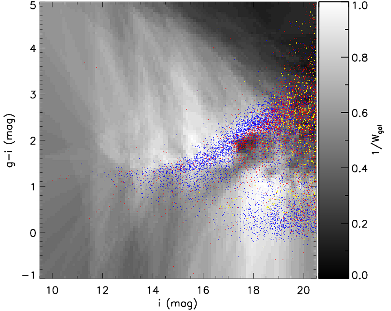
Figure 3. The completeness map in the i -magnitude versus g-i colour plane, used to generate the weight ( w_{\text{gal}} ; shown in sidebar) assigned to each galaxy in constructing the luminosity function. Overlaid blue points are the photometric sample objects above our 2.8 mJy flux limit for which a reliable redshift has been obtained. The overlaid red points are objects for which no spectroscopic follow observation was made. The yellow points represent objects which were observed spectroscopically but a reliable redshift could not be determined. The structure in the completeness map, such as the low completeness for faint objects with g-i colours of \sim 1-2 mag, is mostly the result of targeting completeness in the constituent surveys and demonstrates the importance of constructing our completeness estimates in this plane.
