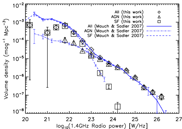
Figure 5. The radio luminosity function for our 0.005 < z < 0.3 redshift bin ( diamonds ). Also, plotted the luminosity function separated into radio AGN ( triangles ) and star-forming radio galaxies ( squares ). The star-forming galaxies outnumber the AGN below P_{1.4\text{GHz}} \sim 10^{23} \text{ W Hz}^{-1} but contribute very little to the number density at higher radio luminosities. Also shown is the radio luminosity functions from Mauch & Sadler (2007) for all sources ( solid blue line ), radio AGN ( dot-dashed blue line ) and radio star-forming galaxies ( dashed blue line ).
