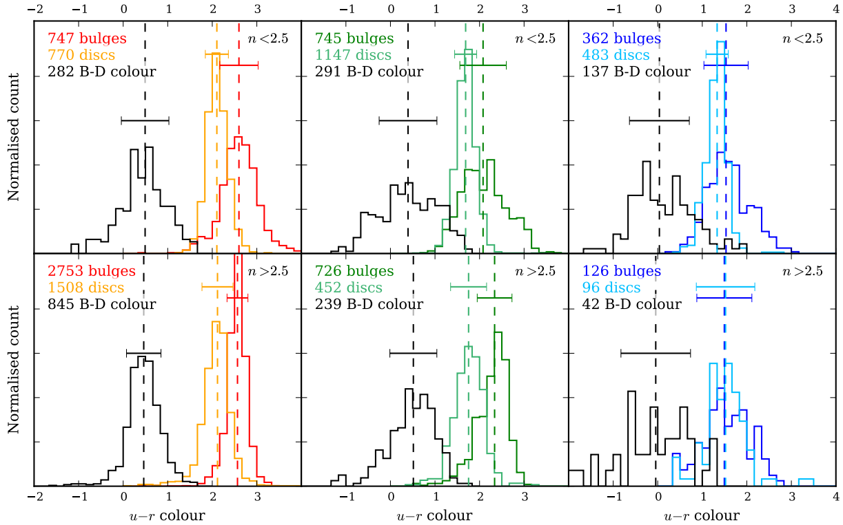
Figure 10. Normalised histogram showing the relative colour distributions of the bulges and discs of a volume-limited sample of M_r < -21.2, z < 0.3 galaxies, binned by Sérsic index and overall galaxy colour, defined as follows: u - r > 2.1 = \text{red} , 1.6 < u - r < 2.1 = \text{green} , u - r < 1.6 = \text{blue} . The B - D colour (i.e. the difference between the u - r colour of the bulge and the u - r colour of the disc within a given galaxy) is plotted in black, with negative values indicating a redder disc than bulge, and positive values indicating a redder bulge than disc. The median B - D colour is plotted as a vertical black dashed line, and the standard deviation of each sample is plotted in the corresponding colour. See table 2 for exact values. Bulges are generally redder than their overall discs, and this colour difference correlates with the overall colour of the galaxy; the bluer the galaxy, the closer the colours of these two components.
