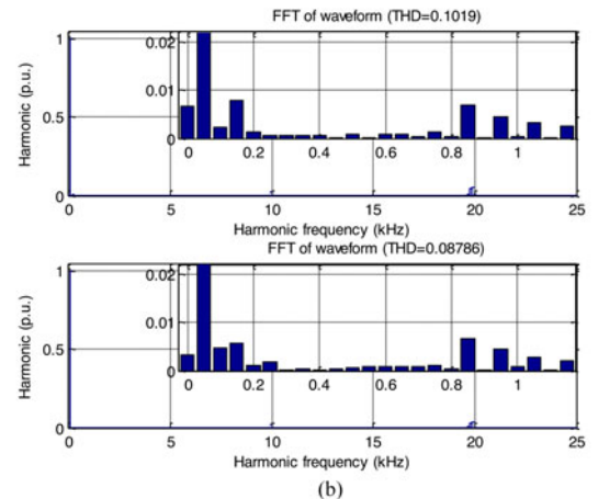
Fig. 18. Asymmetrical six-phase machine in V2G mode: (a) grid voltage v_g , grid current i_g , machine current i_a , and battery charging current i_L ; (b) spectra of grid current i_g (upper graph) and machine current i_a (lower graph).
