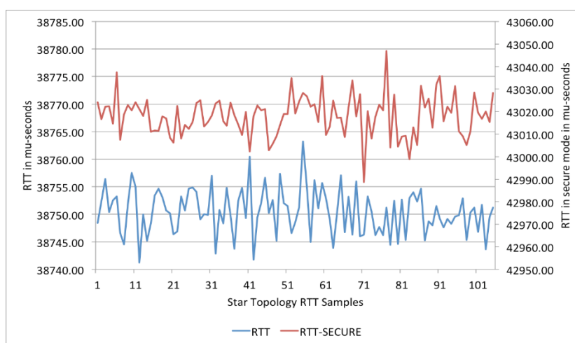
Figure 10. RTT from L-SM to NOC in a star topology (one hop).
