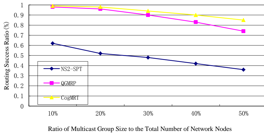
Fig. 9 Comparison of multicast routing success rates over CERNET2 Topology.
