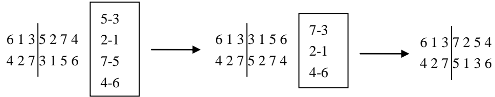
Fig. 6 Partially mapped crossover.
