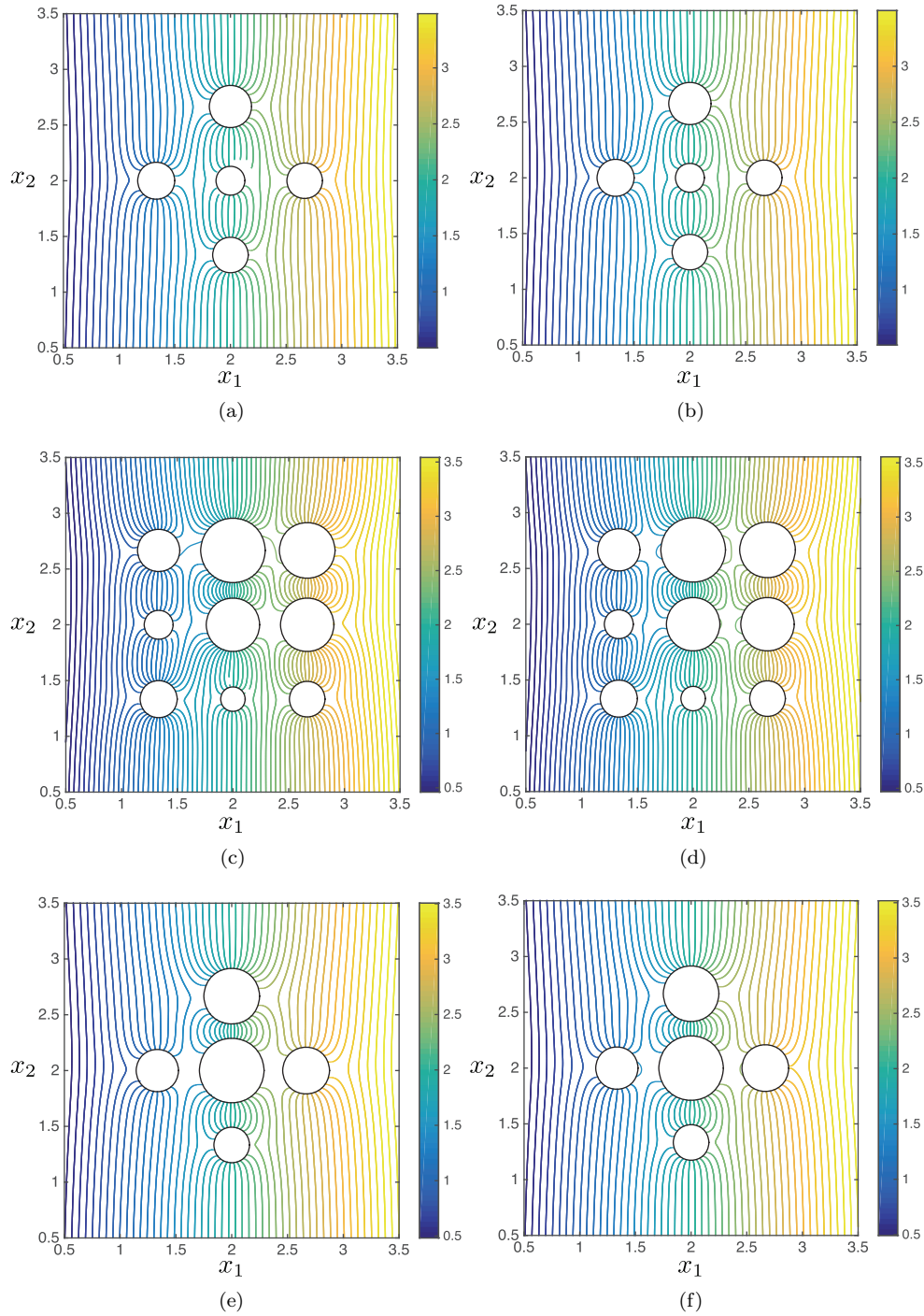
FIG. 4. Figures 4(a), 4(c), and 4(e) show contour plots of the total displacement |\mathbf{u}_N| produced along various planes intersecting the cloud of Figure 3 using data from COMSOL. Figures 4(b), 4(d), and 4(f) show the computations produced by the formula in (7.10) on the same planes. Computations have been carried out along the plane defined by x_3 = 4/3 in Figures 4(a) and 4(b), x_3 = 2 in Figures 4(c) and 4(d), and x_3 = 8/3 in Figures 4(e), and 4(f).
