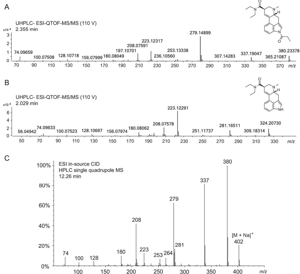
38 Comparison of electrospray ionization single and tandem mass spectra. A: quadrupole time of flight tandem 39 mass spectrum (QTOF-MS/MS) of 1-propionyl-d-LSD (1P-LSD). B: ESI-QTOF-MS/MS of LSD. C: in-source 40 CID spectrum of 1P-LSD under single quadrupole mass spectrometry conditions. 41 190x178mm (300 x 300 DPI)
