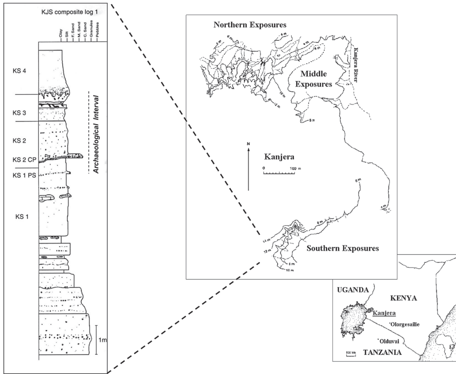
Fig. 1 - The location of Kanjera in southwestern Kenya and of the Southern Exposures at Kanjera where the Oldowan occurrences are found. The composite stratigraphic log shows the basal three beds of the Southern Member of the Kanjera Formation (from oldest to youngest KS-1 to KS-3) and the base of KS-4. Spatially associated artifacts and fossils are found as diffuse scatters and also in more vertically discrete concentrations from the top of KS-1 through KS-3, with KS-2 providing the bulk of the archaeological sample. After Lemorini et al. (2014), Figure 1.
