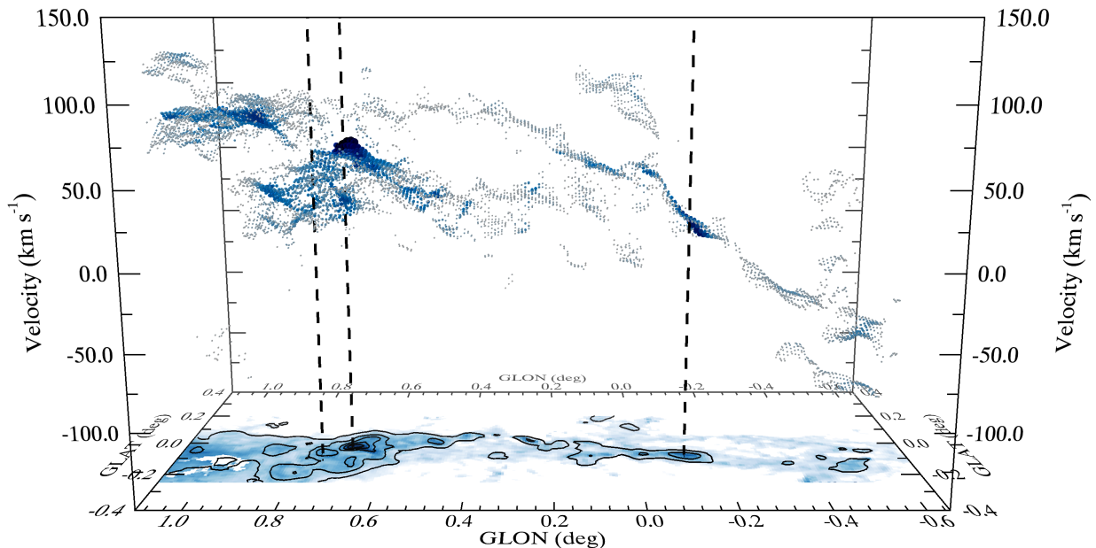
Figure 6. A position-position-velocity (PPV) diagram highlighting the large-scale kinematic structure of the CMZ. Each pixel denotes the location and centroid velocity of a Gaussian component identified in HNC emission and extracted using Scouse. The size (from small to large) and colour (from light to dark) of each data point is proportional to the peak intensity of the corresponding spectral component. At the base of the plot, in logarithmic colour-scale, is the Herschel -derived molecular hydrogen column density map (Battersby et al., in prep.). Column densities range from 10^{22} – 10^{24} \text{cm}^{-2} . Overlaid are contours highlighting the distribution of HNC integrated emission. Contour levels are, 5, 25, 45, 65, and 85 per cent of peak (integrated) emission (cf. Figure 4). The three vertical dotted lines refer to the locations P1, P2, and P3, also highlighted in Figure 4 (the corresponding spectra of which are shown in Figure 3). A movie that shows this figure in 3-D is available in the online supplementary material.
