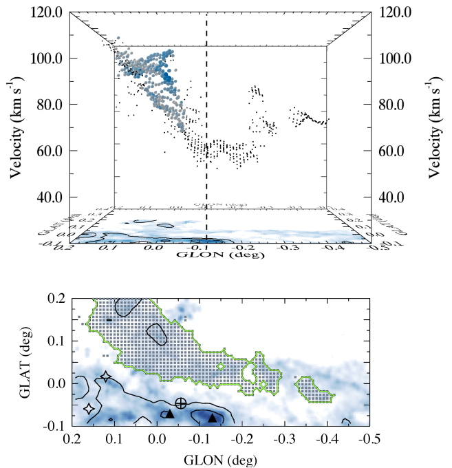
Figure 11. Top panel: A PPV image of ‘‘Arm III’’ (Sofue 1995; also known as the ‘‘polar arc’’ in Bally et al. 1988, see § 4.3.1). The coloured data points are equivalent to those presented in Figure 10. Bottom panel: A map indicating the spatial distribution of the data points shown in the PPV diagram. The green contour and symbols are equivalent to those in Figure 9. The background image and contours in both panels are equivalent to those in Figure 6.
