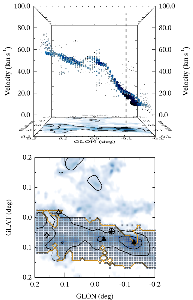
Figure 15. Top panel: A PPV diagram of the molecular gas distribution between -0^{\circ}2 < l < 0^{\circ}2 and -0^{\circ}15 < b < 0^{\circ}05 in position and 0.0 \text{ km s}^{-1} < v_{\text{LSR}} < 60.0 \text{ km s}^{-1} in velocity. This region incorporates several massive molecular clouds, including the 20 \text{ km s}^{-1} and 50 \text{ km s}^{-1} clouds, and GCM 0.11–0.11. The data points have equivalent meaning to those presented in Figure 10. Bottom panel: Highlighting the distribution of data points in the top panel. The background image and contours in both panels are equivalent to those in Figure 6.
