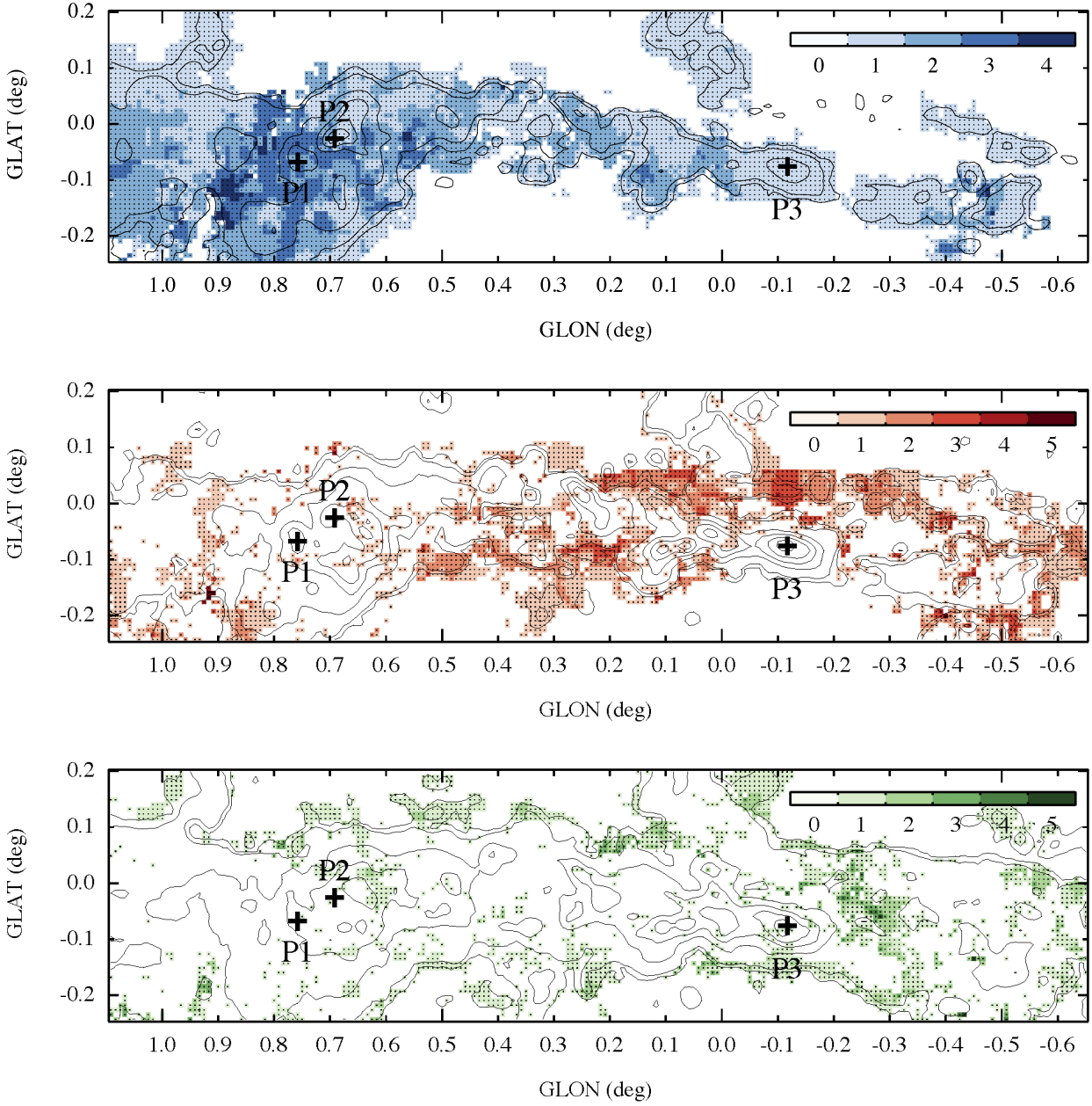
Figure A2. Illustrating the result of the merger process. The top panel is equivalent to Figure 4. Each coloured pixel refers to a location with a corresponding best-fit solution. Each pixel is colour-coded according to the number of velocity components identified at that location. The central and bottom panels are the same but for the \text{N}_2\text{H}^+ and HNC data, respectively (note that only components selected during the merging process outlined in Appendix A are shown). Contours in all cases show the integrated intensity of the respective molecular line. Contour levels are, 1, 5, 25, 45, 65, and 85 per cent of peak (integrated) emission.
