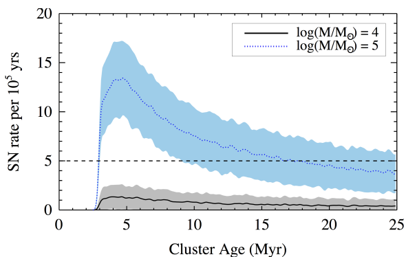
Figure 14. Plotting the estimated supernova rate (per 10^5 yrs) versus age for two star clusters of masses M_{cl} = 10^4 M_{\odot} (black) and 10^5 M_{\odot} (blue), respectively. The shaded region represents the standard deviation in the supernova rate over 100 runs of the simulation (for a more in-depth description of the methodology, please refer to Appendix B). The horizontal dashed line indicates the supernova rate inferred by Tanaka et al. (2014) to explain the expansion motion of a shell-like feature observed in velocity-integrated emission maps towards the Sgr C molecular cloud complex ( \sim 5 \times 10^{-5} \text{ yr}^{-1} ). As is indicated, a star cluster of M_{cl} > 10^4 M_{\odot} would be required to reproduce the supernova rate of Tanaka et al. (2014).
