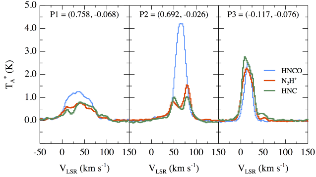
Figure 3. Selected spectra from the Mopra CMZ survey (the positions of these spectra are highlighted with ‘+’ symbols in Figure 4). The spectra of three molecular lines are shown within each panel, HNCO (blue), \text{N}_2\text{H}^+ (red), and HNC (light green). P1 and P2 are close to the Sgr B2 region (with P2 representing the location of peak HNCO emission), and P3 represents the peak in HNCO emission at negative longitudes (at \sim the location of the 20 \text{ km s}^{-1} cloud). Note the double-peaked profiles (possibly indicating self-absorption) in all but the HNCO line at P2. HNCO is selected as our primary tracer of the kinematics within the CMZ.
