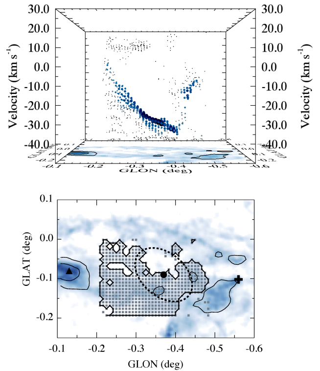
Figure 13. Top panel: A PPV diagram of the molecular gas distribution between -0^{\circ}5 < l < -0^{\circ}2 and -0^{\circ}2 < b < 0^{\circ}0 in position and -40.0 \text{ km s}^{-1} < l < 20.0 \text{ km s}^{-1} in velocity, as part of the Sgr C molecular cloud complex. The data points have equivalent meaning to those presented in Figure 10. Bottom panel: Highlighting the distribution of data points in the top panel. The filled black circle and dashed black ellipse indicate the centre position and physical extent of a shell of molecular emission reported in Tanaka et al. (2014) and discussed in § 4.3.2. The background image and contours in both panels are equivalent to those in Figure 6.
