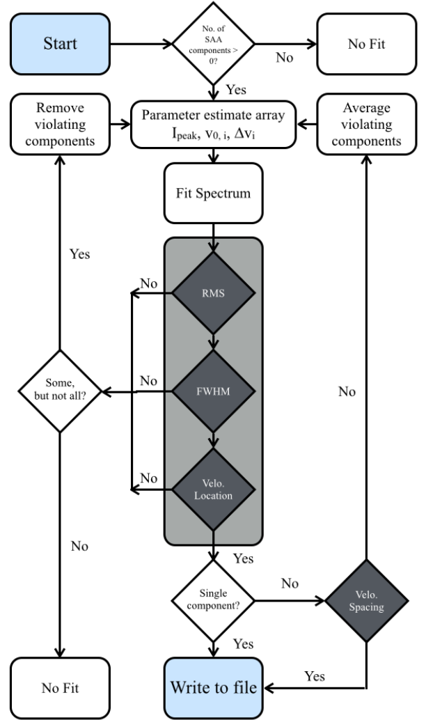
Figure 2. A flowchart illustrating the algorithm governing stage 3 of the SCOUSE fitting routine (§ 3.1.3). Decisions are indicated by diamonds, with tolerance-dependent decisions shaded in grey.
