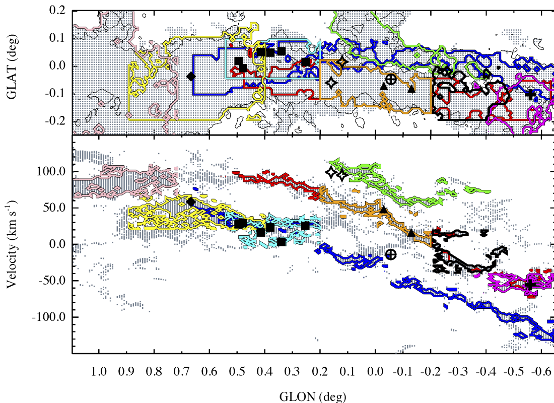
Figure 9. Combining molecular gas kinematics at 3 mm. The top panel depicts the spatial distribution ( l, b ) of dense gas within the CMZ, including HNC, N_2H^+ , and HNC. Each pixel denotes a location with a corresponding best-fitting solution. The single contour refers to a molecular hydrogen column density of 10^{22} \text{ cm}^{-2} (Battersby et al., in prep.). The bottom panel is a position-velocity ( l, v_{\text{LSR}} ) diagram with each pixel referring to the Galactic longitude and centroid velocity of a spectral component. The black circle with a plus denotes the location of Sgr A*, and the open stars represent the Arches and Quintuplet clusters (the Arches cluster has the smallest projected distance from Sgr A*). Additionally, the locations of prominent molecular clouds are overlaid. In order of increasing Galactic longitude (from right to left): The Sgr C complex (black plus); the 20 \text{ km s}^{-1} and 50 \text{ km s}^{-1} clouds (black upward triangles); G0.256+0.016 (black square); Clouds B-F (black squares); The Sgr B2 complex (black diamond). The position and velocity limits of the molecular clouds can be found in Table 3. The coloured contours highlight some of the most prominent PPV-structures. The blue contour shows “Arm I” (Sofue 1995; also known as the “negative velocity filament” in Bally et al. 1988). The red contour shows “Arm II” (Sofue 1995). Both of these structures, as well as their possible connection to the PPV-structure highlighted by the pink contour, are discussed in § 4.3.1. The green contour highlights “Arm III” (also known as the “Polar arc” in Bally et al. 1988) and it is also discussed in § 4.3.1. The magenta and black contours refer to molecular gas associated with the Sgr C complex (see § 4.3.2 and Figures 12 and 13, respectively). The orange contour shows the 20 \text{ km s}^{-1} and 50 \text{ km s}^{-1} clouds (see § 4.3.3). The cyan contour highlights the “dust ridge” (Lis et al. 1994, 2001; see § 4.3.4 and Figure 16). The yellow contour highlights the Sgr B2 cloud complex (see § 4.3.5 and Figure 17). Note that there is overlap in the data associated with several of these PPV-structures since they are not all independent. This is particularly evident throughout Arm II, which also incorporates data associated with the 20 \text{ km s}^{-1} and 50 \text{ km s}^{-1} clouds and the Sgr C molecular cloud complex.
