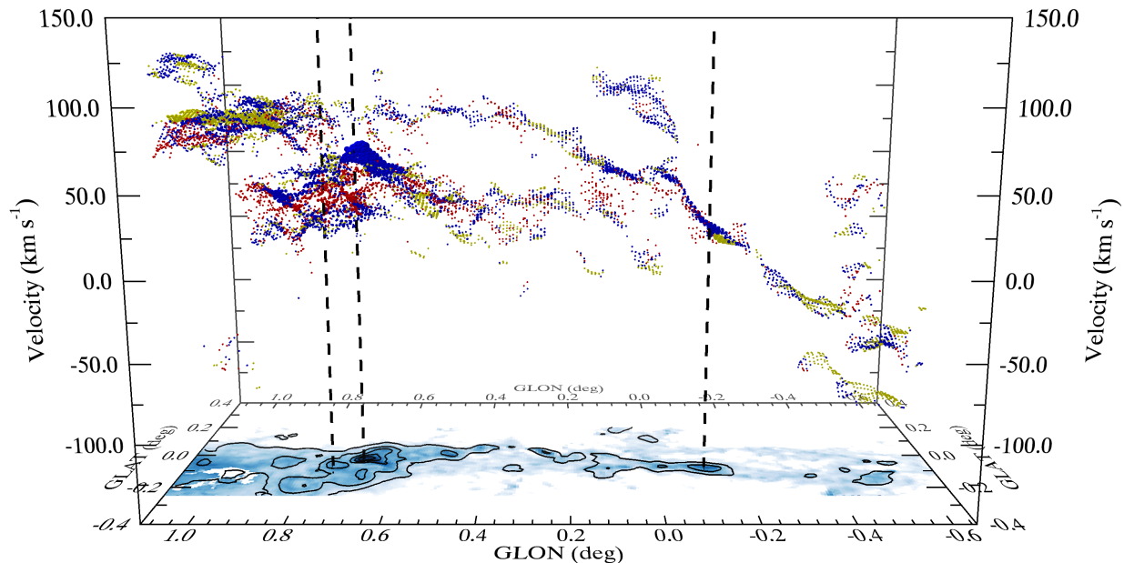
Figure 8. The same as Figure 6. However, each pixel is now colour-coded according to specific ranges in velocity dispersion (see § 4.2.2 for more information on the selection of these ranges). Yellow: 2.6 \text{ km s}^{-1} < \sigma < 7.4 \text{ km s}^{-1} ; Blue: 7.4 \text{ km s}^{-1} < \sigma < 13.3 \text{ km s}^{-1} ; Red: 13.3 \text{ km s}^{-1} < \sigma < 53.1 \text{ km s}^{-1} . Note the contrast in velocity dispersion between the Sgr B2 (where \sim 45 per cent of the high-dispersion gas lies) and Sgr C (which predominantly exhibits low- or intermediate dispersion gas) molecular cloud complexes situated at \{l, b, v_{\text{LSR}}\} \sim \{0^{\circ}70, -0^{\circ}05, 60 \text{ km s}^{-1}\} and \sim \{-0^{\circ}50, -0^{\circ}10, -55 \text{ km s}^{-1}\} , respectively.
