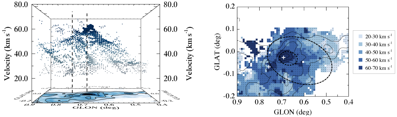
Figure 17. Left: A PPV diagram of Sgr B2. Only the HNC0 solutions are shown to avoid confusion caused by the self-absorption observed in the \text{N}_2\text{H}^+ and HNC spectral line profiles (see § 3.2). The data points are colour-coded according to five different velocity ranges (note the key on the right-hand side of the figure): 20\text{--}30\text{ km s}^{-1} ; 30\text{--}40\text{ km s}^{-1} ; 40\text{--}50\text{ km s}^{-1} ; 50\text{--}60\text{ km s}^{-1} ; 60\text{--}70\text{ km s}^{-1} . As with Figure 6, the size of each data point is proportional to the peak intensity of the corresponding spectral component. The vertical dashed lines are equivalent to those in Figure 6 and refer to positions P1 and P2 (the corresponding spectra of which are shown in Figure 3). Right: A map showing the spatial distribution of the data points shown in the left panel. The black contours are equivalent to those presented in Figure 4. The colours are equivalent to those in the left panel. The black dot-dashed ellipse refers to the location of the ring of emission identified by Bally et al. (1987) between 20\text{--}40\text{ km s}^{-1} . The black dashed ellipse highlights the location of the “hole” in ^{13}\text{CO} (1-0) emission discussed by Hasegawa et al. (1994). These images reveal the “cone-like” PPV-structure of Sgr B2 discussed in § 4.3.5. This illustrates how a conical PPV-structure can lead to the perception of shells (and corresponding holes) in velocity-integrated emission maps.
