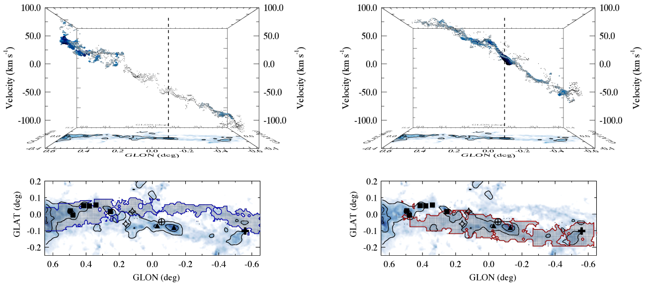
Figure 10. Top panels: PPV diagrams of the two extended features noted in the \{l, v_{\text{LSR}}\} projections of Figure 9 and discussed in more detail in § 4.3.1. The coloured data points are equivalent to those presented in Figure 6. Black data points highlight the \{l, b, v_{\text{LSR}}\} location of both the \text{N}_2\text{H}^+ and HNC components. Bottom panels: Maps indicating the spatial distribution of the data points shown in the top panels. The left panels show “Arm i” (Sofue 1995; also known as the “negative velocity filament” in Bally et al. 1988). Kruijssen et al. (2015) argue that the data points shown in the left panels are distributed into two physically independent structures that are situated on the near- and far-sides of the Galactic centre, respectively (rather than a single spiral arm; Sofue 1995). The right panels depict “Arm ii” of Sofue 1995. We discuss how the structures in this figure may contribute to the 3-D structure of the CMZ in § 4.4). The blue and red contours, and black symbols are equivalent to those shown in Figure 9. The background image and contours in all panels are equivalent to those in Figure 6.
