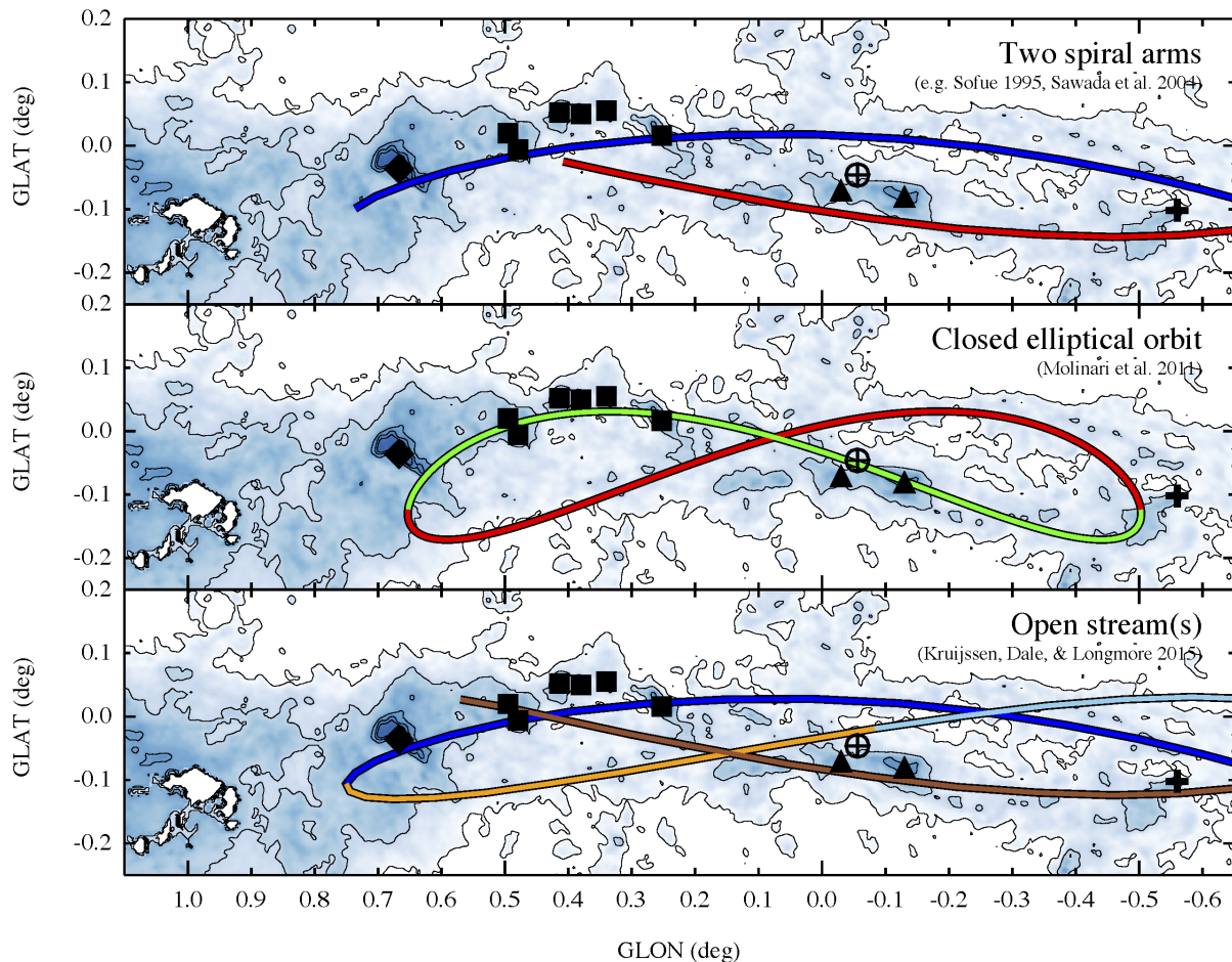
Figure 18. The Herschel -derived molecular hydrogen column density map of the CMZ (Battersby et al. in prep.) overlaid with three different interpretations of the 3-D structure of the CMZ (as they would appear in projection on the sky; \{l, b\} ). The top panel depicts the interpretation that the gas and dust distribution of the CMZ is organised into two prominent spiral arms (see § 4.4.1). “Arm I” (blue) is situated on the near-side of the Galactic centre, whereas “Arm II” (red) is situated on the far-side. The two spiral arms are illustrated in this figure using Streams 1 (Arm II) and 2 (Arm I) of the Kruijssen et al. (2015) orbital solution (note that the physical interpretation of the Kruijssen et al. 2015 orbital solution is fundamentally different from the geometry presented by Sofue 1995, see § 4.4.3). The latitude of these two streams has been altered such that the arms are approximately point symmetric about Sgr A*. The central panel depicts the Molinari et al. (2011) orbital geometry. In this interpretation, the gas and dust follow a closed elliptical orbit around Sgr A* (see § 4.4.2). The green and red portions of the orbit represent the the near and far side (when viewed in projection), respectively. The bottom panel depicts the dynamical orbital solution of Kruijssen et al. (2015). In this model, material follows an open eccentric orbit around Sgr A* (see § 4.4.3). The colours in this final panel refer to those presented by Kruijssen et al. (2015). Streams 1, 2, 3, and 4 appear in brown, blue, orange, and cyan, respectively. The point-of-interest markers are identical to those presented in the top panel of Figure 9.
