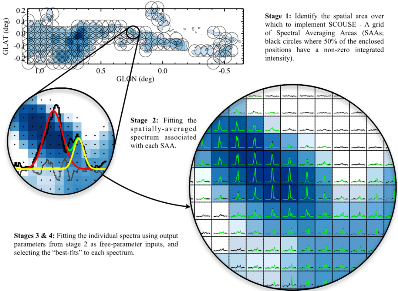
Figure 1. A schematic figure highlighting the main stages of SCOUSE. All data shown correspond to the HNC0 4(0,4)-3(0,3) transition from the Mopra CMZ survey (Jones et al. 2012). The top left image displays a contour map of the integrated emission of HNC0 throughout the CMZ and refers to stage 1 (see § 3.1.1 for details). The filled contours represent 1, 5, 25, 45, and 65 per cent of peak (integrated) emission ( \sim 122 \text{ K km s}^{-1} ). Black circles are the SAAs that make up the coverage (regions whereby 50 per cent of the enclosed spectra have non-zero integrated emission). The centre-left image is a close up image of the SAA associated with G0.253+0.016, an IRDC with known kinematic complexity (e.g. Kauffmann et al. 2013; Bally et al. 2014; Johnston et al. 2014; Rathborne et al. 2014a; Mills et al. 2015; Rathborne et al. 2015). The spatially-averaged spectrum taken from this SAA is shown in black. The velocity range displayed is -110.0 \text{ km s}^{-1} < v_{\text{LSR}} < 170.0 \text{ km s}^{-1} . The line profile is dominated by at least two distinct components (the residual spectrum in grey suggests that additional velocity components may be present). The minimisation algorithm MFFIT (Markwardt 2009) finds the best fitting solution to Equation 1, following the insertion of (user-provided) initial estimates for the parameters that describe each Gaussian component (stage 2; see § 3.1.2 for more details). The two Gaussian profiles (seen in red and yellow), and total profile (seen in green), are the result of this process. The bottom-right image represents stages 3 and 4. It depicts the same SAA however, now the resultant fit to each of the pixels marked by black dots in the stage 2 image is displayed. The observed line profiles are the result of applying the algorithm described in Figure 2 (stage 3; see § 3.1.3). Alternative solutions to each composite spectrum are provided from neighbouring SAAs. In this way, the final results are not restricted to two velocity components. Instead, these are the best solutions selected from a sample of overlapping SAAs (stage 4; see § 3.1.4).
