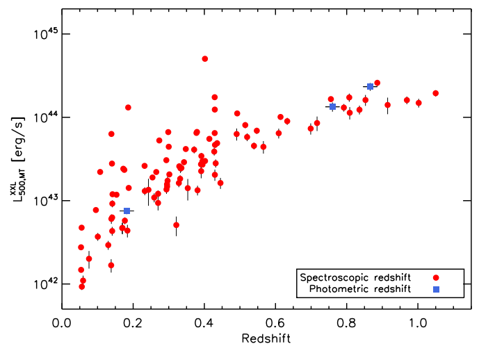
Fig. 5. Distribution of the bright XXL cluster sample in the (z, L_X) vs redshift plane. The luminosity is measured in the [0.5–2] keV band and integrated to r_{500, \text{MT}} . The data show a clear Malmquist bias due to the flux selection combined with volume effects that prevent us from detecting massive (and thus luminous) clusters at low redshift.
